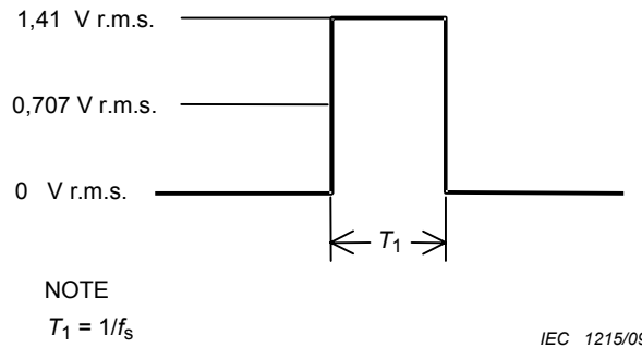
Figure 1 – Analogue test signal waveform
