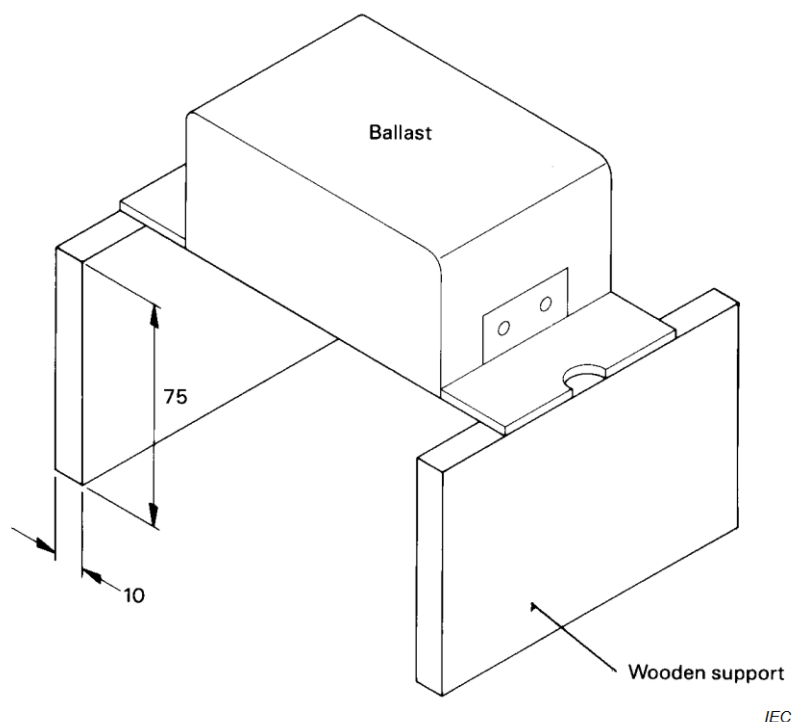
Figure H.1 – Test arrangement for heating test
