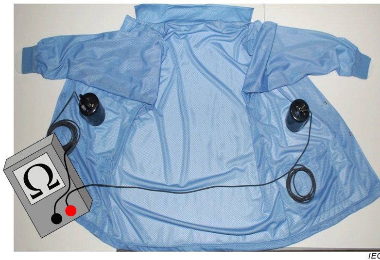
Figure 3 – Test set-up – Resistance point-to-point (panel-to-panel procedure with insulative support surface)
