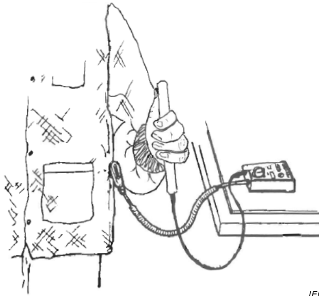
Figure 11 – Test set-up – Groundable static control garment system resistance (groundable garment in combination with a person using a meter and hand-held electrode)
