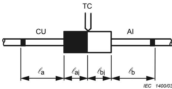
Figure 3b – Through connector
