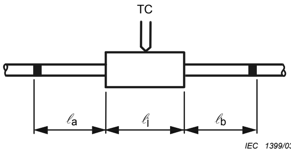
Figure 3a – Reference conductor
