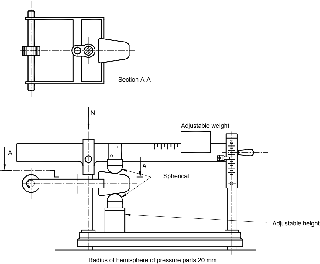
Figure 18 – Pressure apparatus
