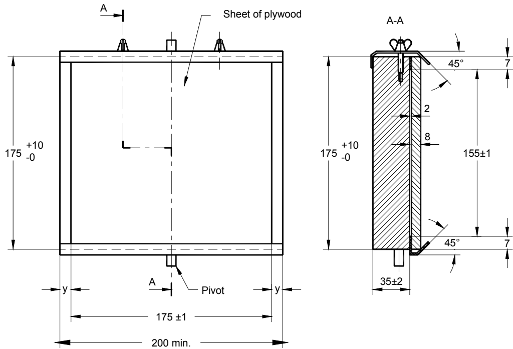
Figure 16 – Mounting support
