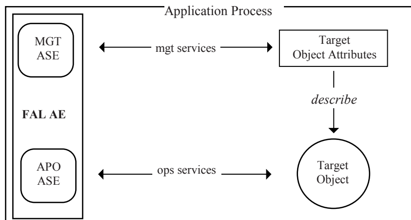
Figure 18 – FAL management of objects
