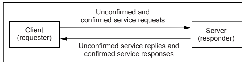
Figure 12 – Client/server interactions
