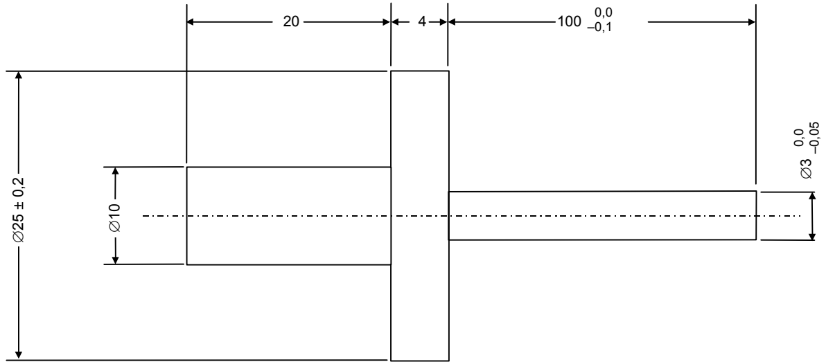
Figure C.4 – 100 mm × 3 mm test pin
