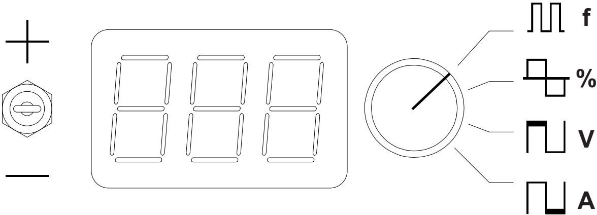
Figure L.8 – Setting pulsing parameters using digital display
