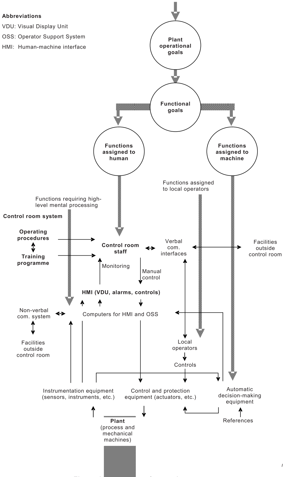
Figure 1 – Overview of control room system
