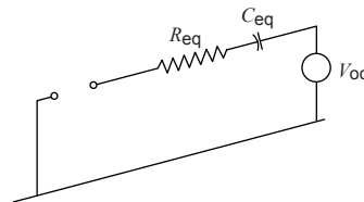
Figure C.8 – Basic circuit for arcing test
