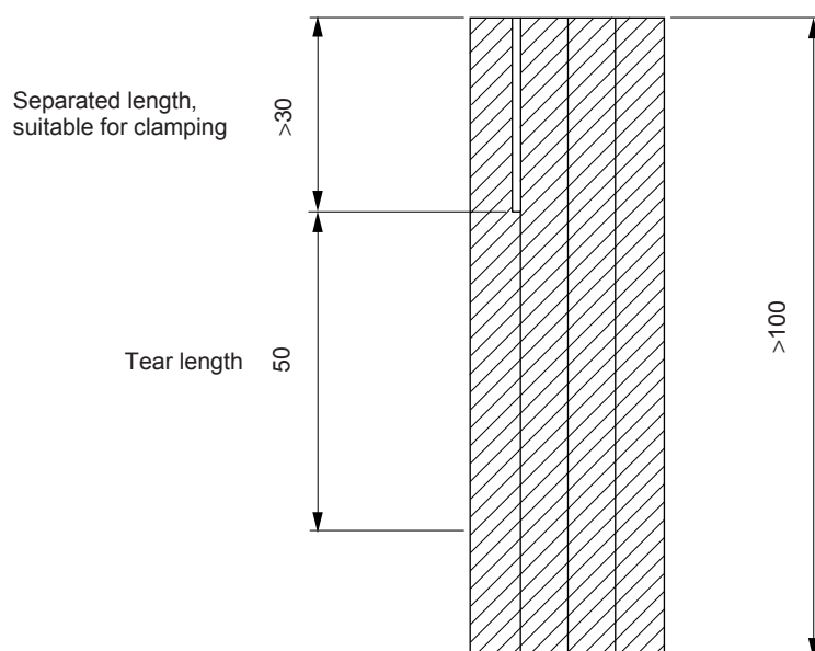
Figure 3 – Sample preparation
