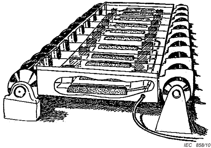
Figure A.5 – Ganged rotating capstan tester
