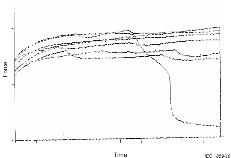
Figure B.1 – Gradual slippage
