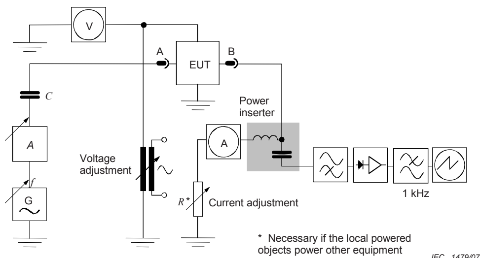
Figure 5 – Test set-up for power injectors
