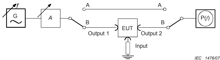
Figure 2 – Test set-up for the measurement of isolation
