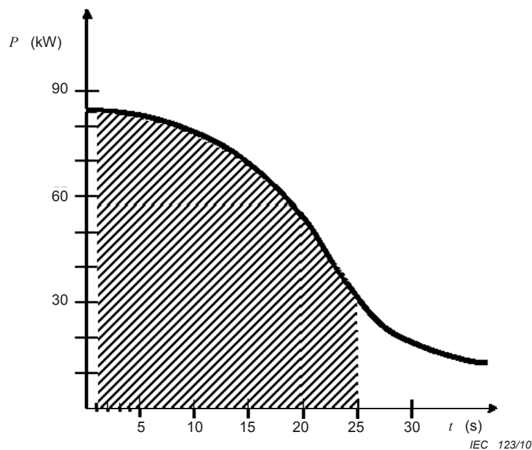
Figure A.1 – Example: SINGLE LOAD RATING chart showing CTSPI calculation area for scan time interval of 1 s to 25 s
