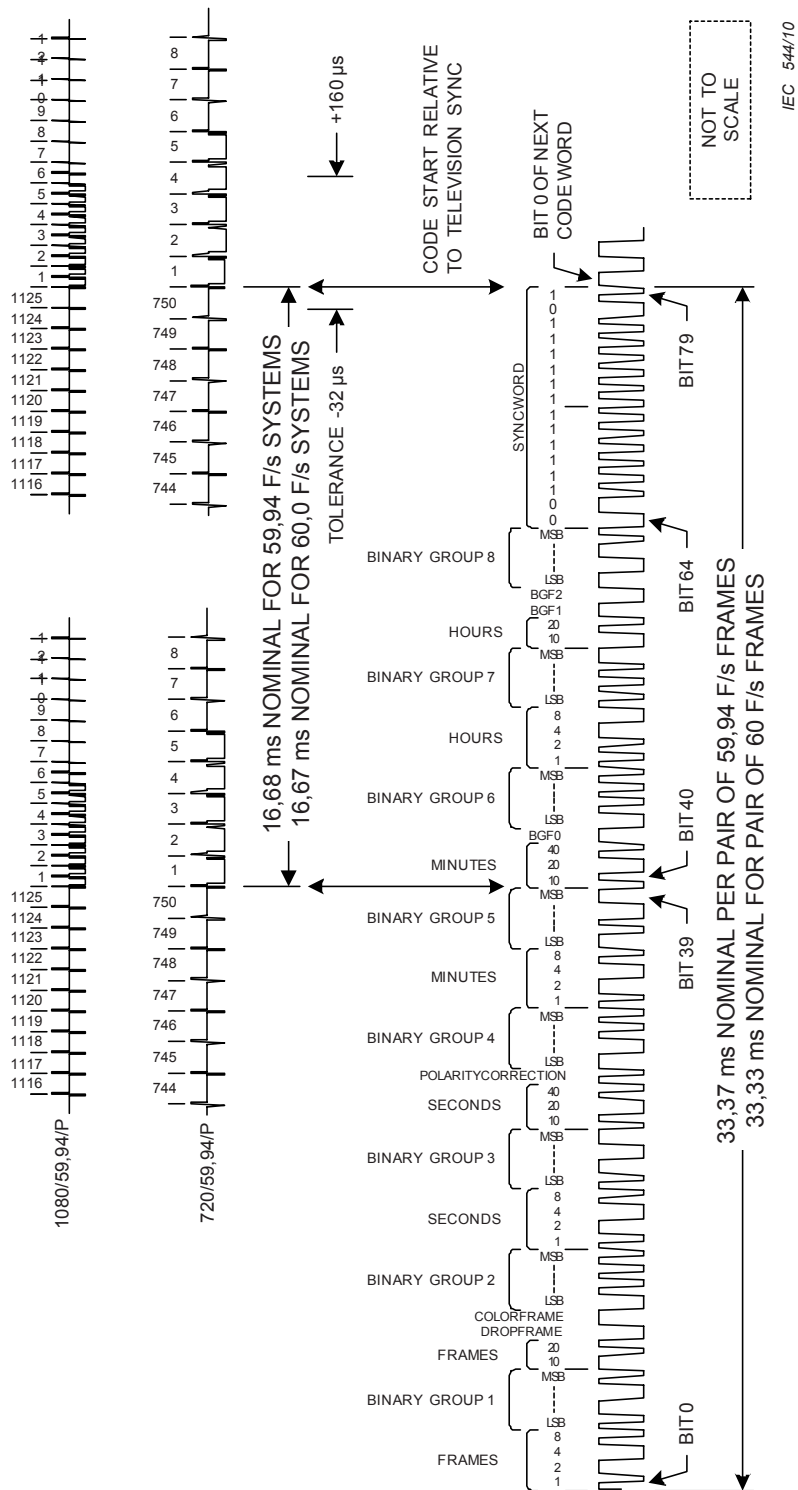
Figure 5 – Linear time code relationship to 59,94 frame progressive video example
