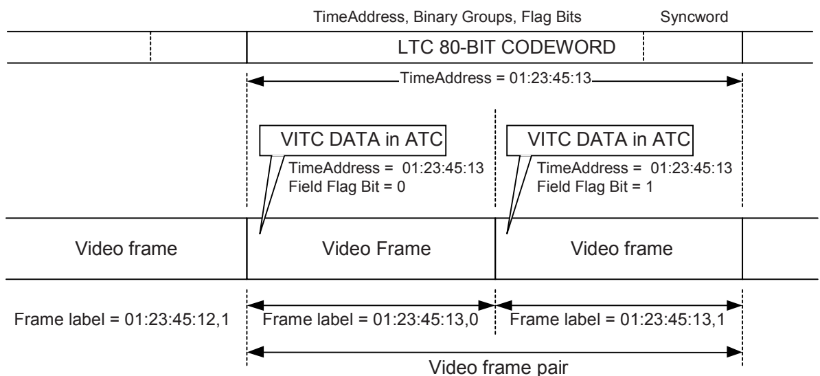
Figure 9 – Example of frame labeling for 50 and 60 frames per second progressive systems
