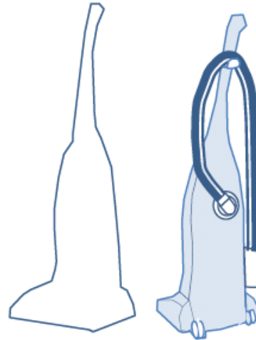
Figure Z.2 – Typical upright vacuum cleaner with secondary hose (contour front and back)
