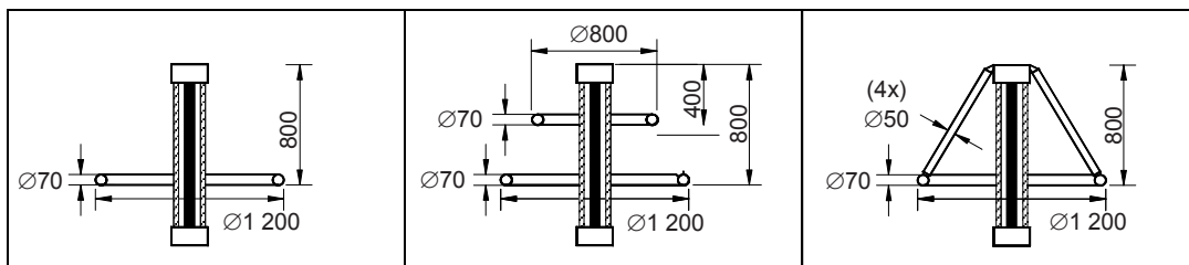
Figure F.3a – Simplified model of multi-unit arrester
