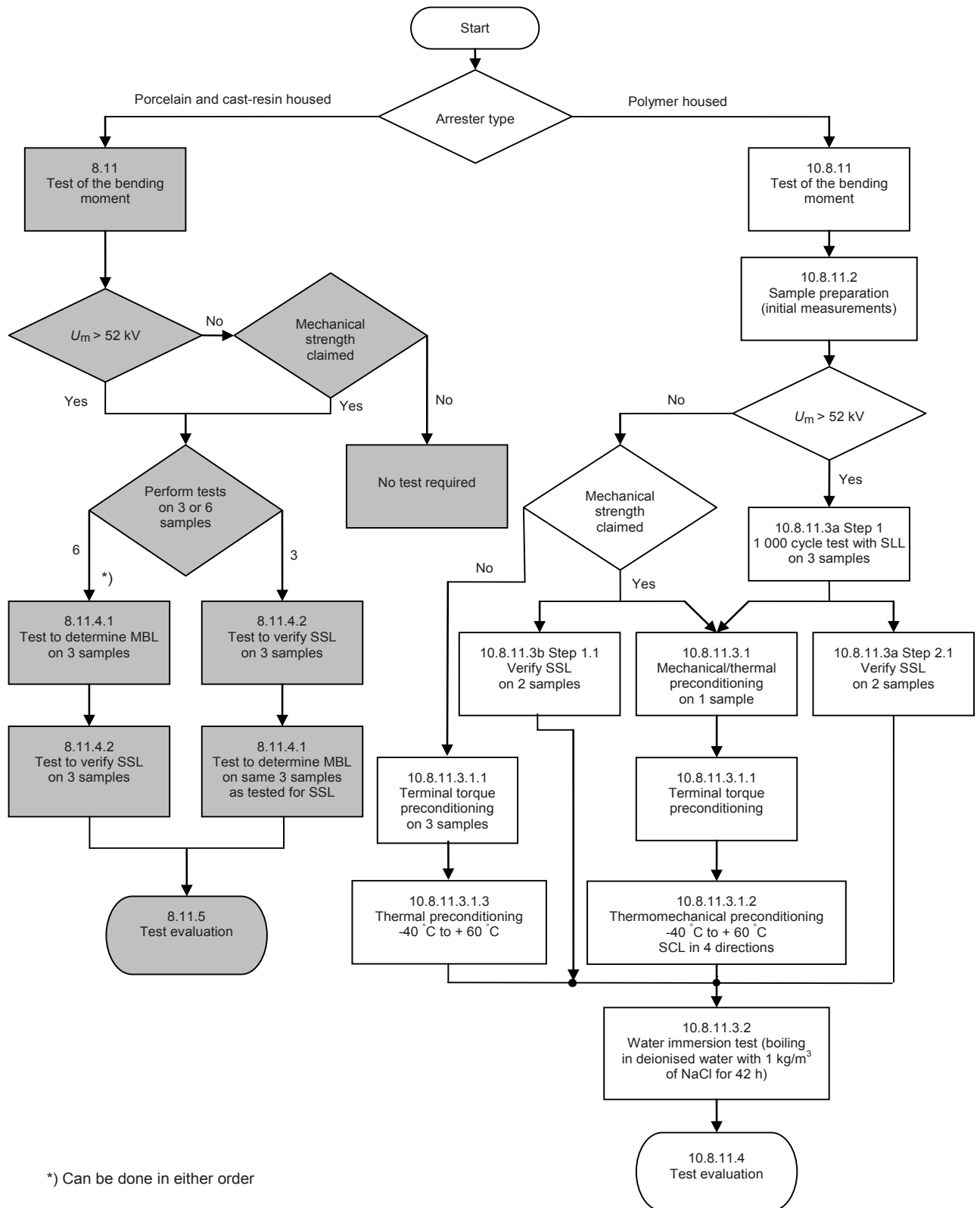
Figure G.5 – Flow chart of bending moment test procedures
