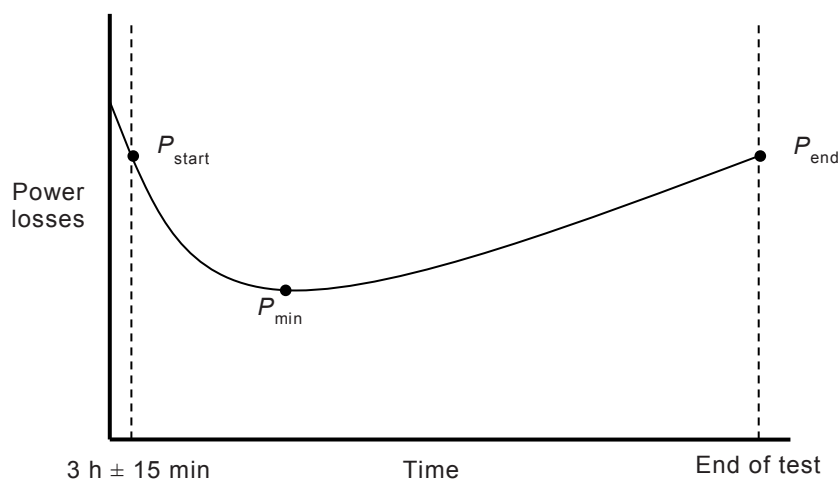
Figure 1 – Illustration of power losses versus time during long term stability test
