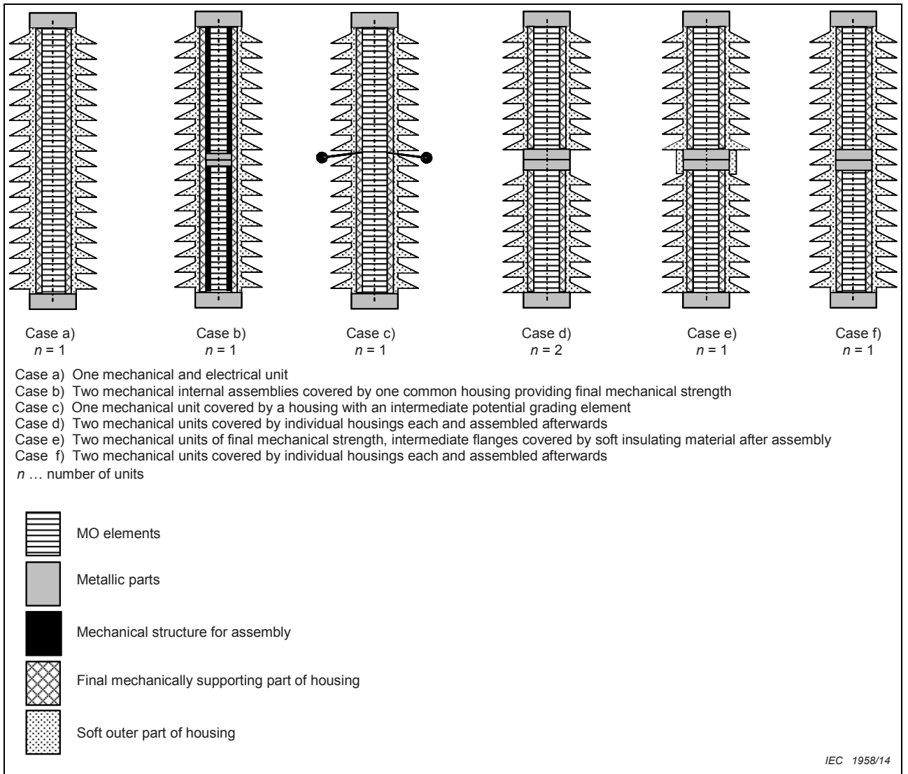
Figure 5 – Examples of arrester units
