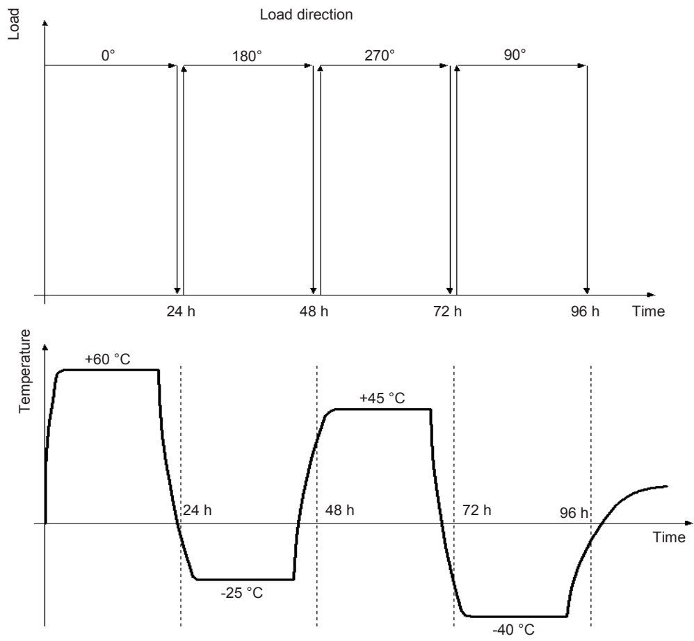
Figure 11 – Thermomechanical test
