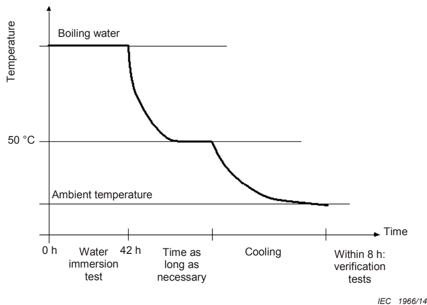
Figure 13 – Water immersion
