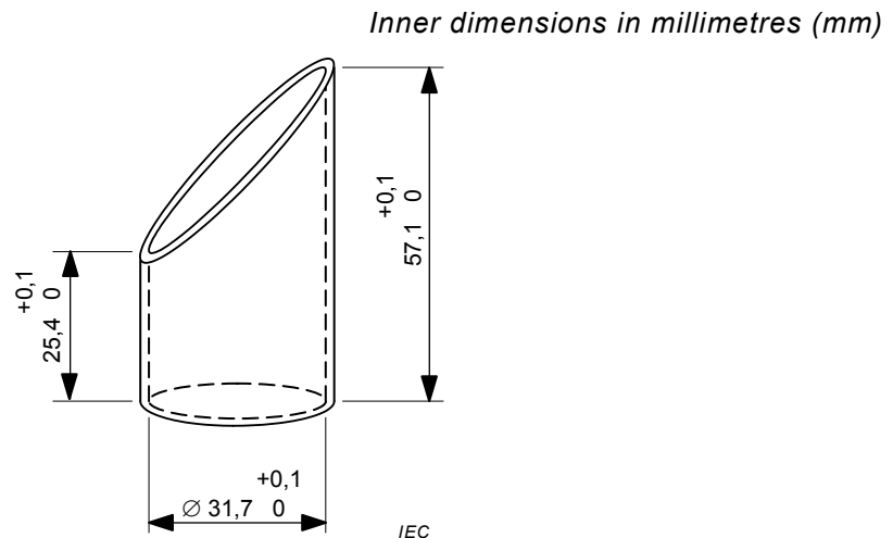
Figure 1 – Ingestion gauge
