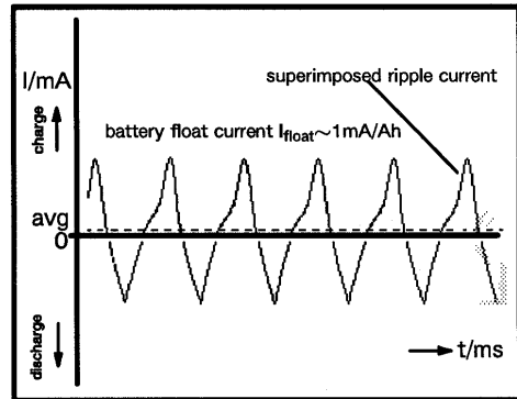
Figure A.5 - Magnified battery float charge with superimposed ripple current
