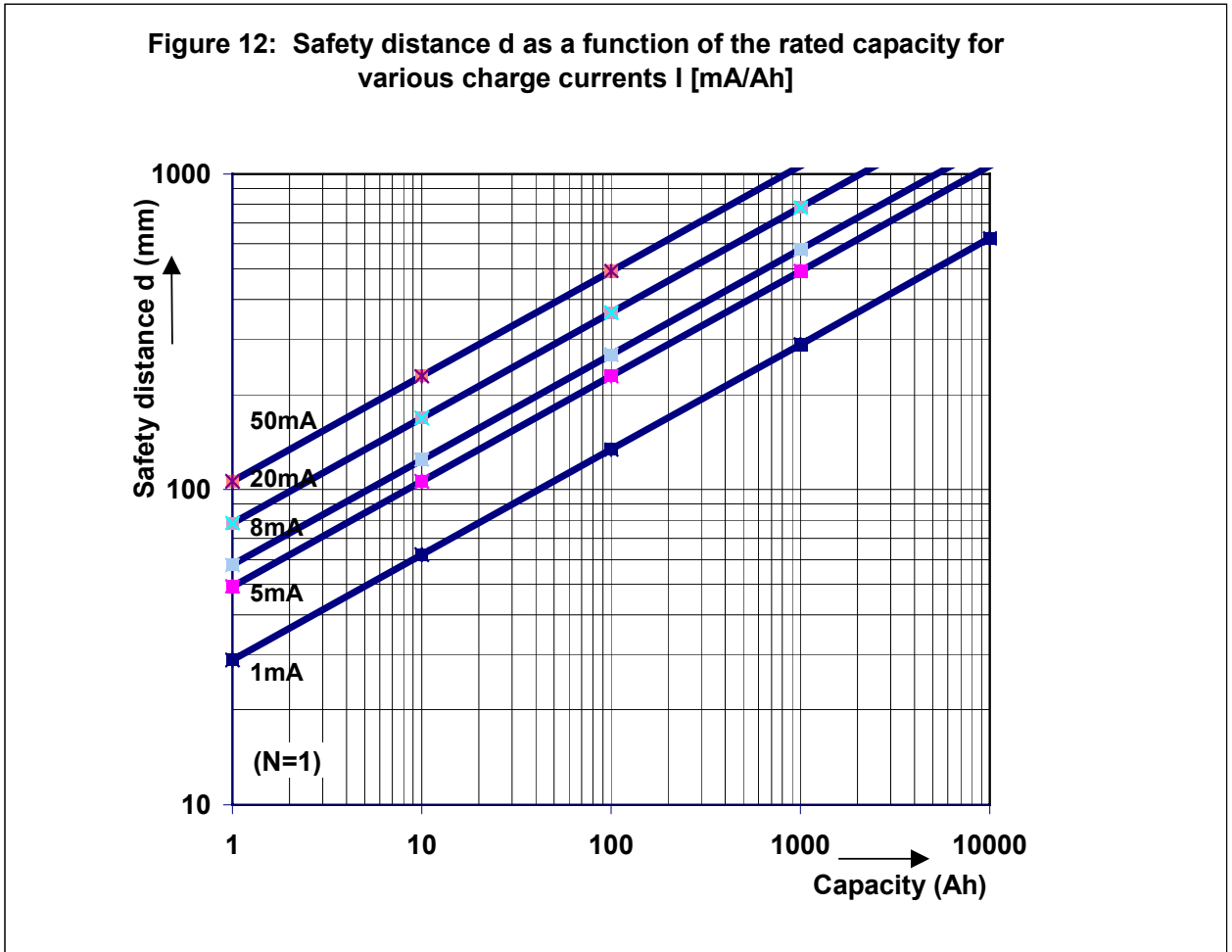
Figure B.1 - Safety distance d as a function of the rated capacity for various charge currents I [mA/Ah]
