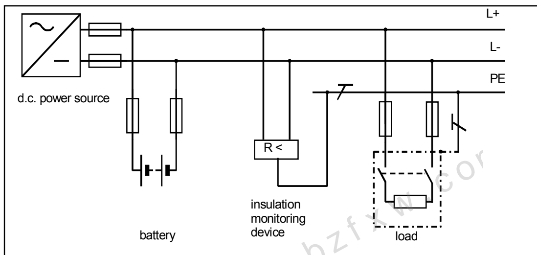
Figure 4 - IT system
