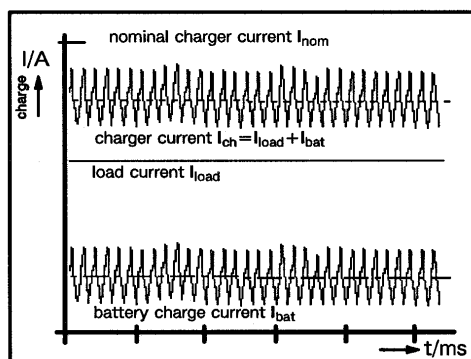
Figure A.2 - The charger supplies the full current to the load and to the battery
