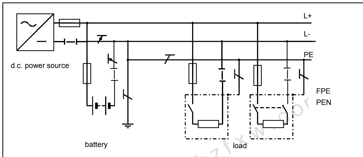
Figure 1 - TN system with separate protective conductor (PE) in the entire system (TN-S network)
