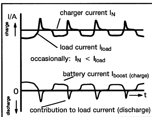
Figure A.6 - The charger does not supply the full current to the load and to the battery
