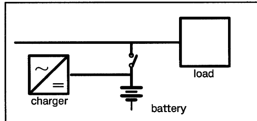
Figure A.8 - Response mode operation
