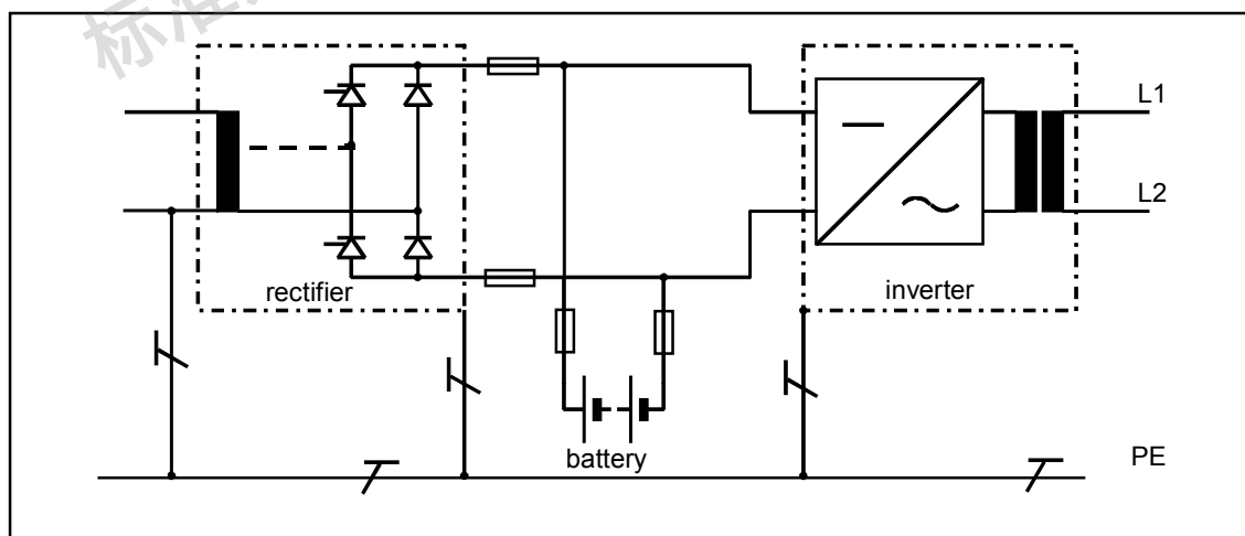
Figure 5 - Convertors with intermediate DC circuit (IT-System) (Example)
