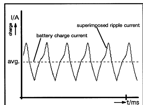
Figure A.3 - Magnified battery charge with superimposed ripple current
