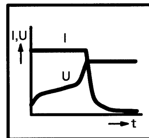
Figure A.10 - Time dependant characteristic of current I and voltage U
