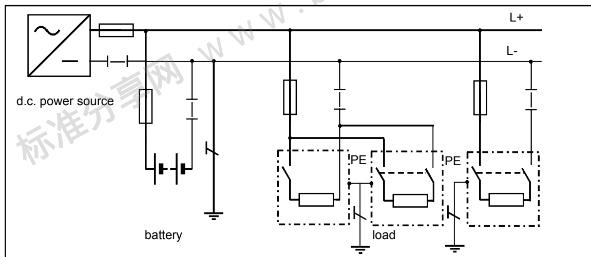
Figure 3 - TT system
