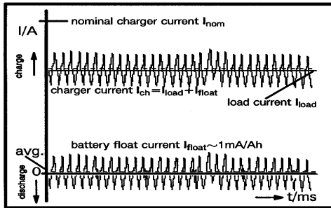
Figure A.4 - The charger supplies the full current to the load and to the battery
