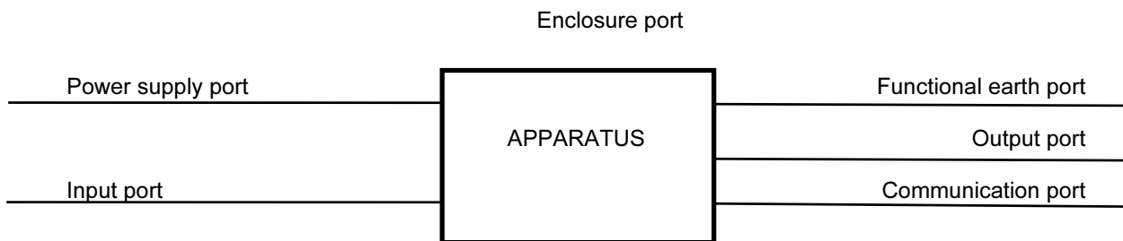
Figure 1 - Ports for measuring relays and protection equipment
