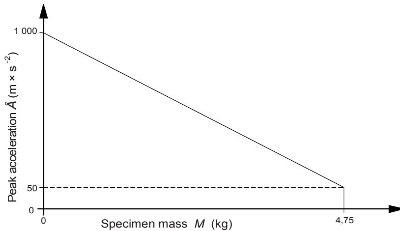
Figure 1 – Graph showing peak acceleration vs. specimen mass
