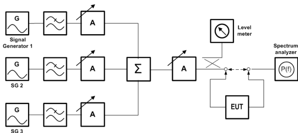
Figure 11 - Measurement set-up for internal immunity test
