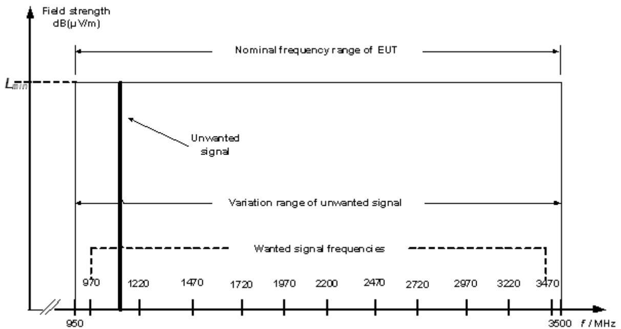
Figure 9 - Frequency allocation for in-band immunity measurement of active equipment with nominal upper frequency limit \leq 1\ 000 MHz
