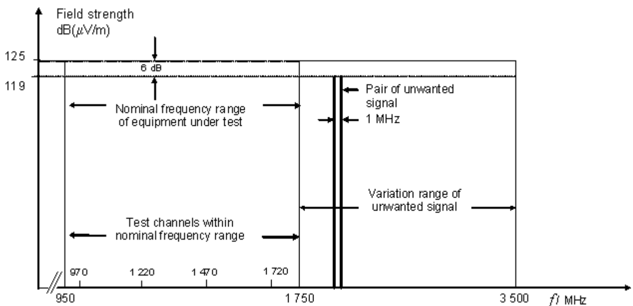
Figure 7 - Frequency allocation for out-of-band immunity measurement of active equipment with nominal upper frequency limit \leq 1\,000 MHz
