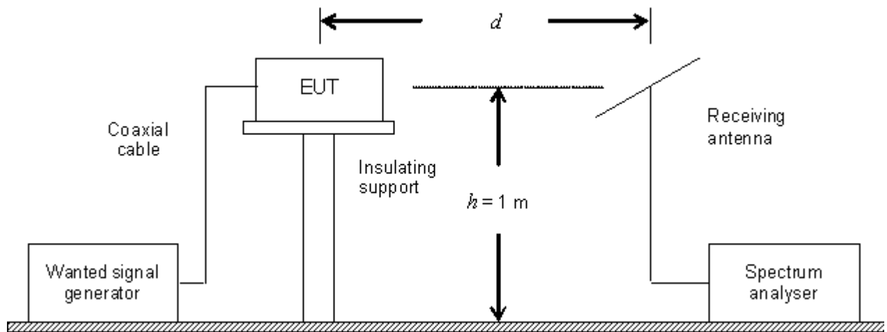
Figure 5 - Measurement set-up for the "substitution" radiation method – First measurement step
