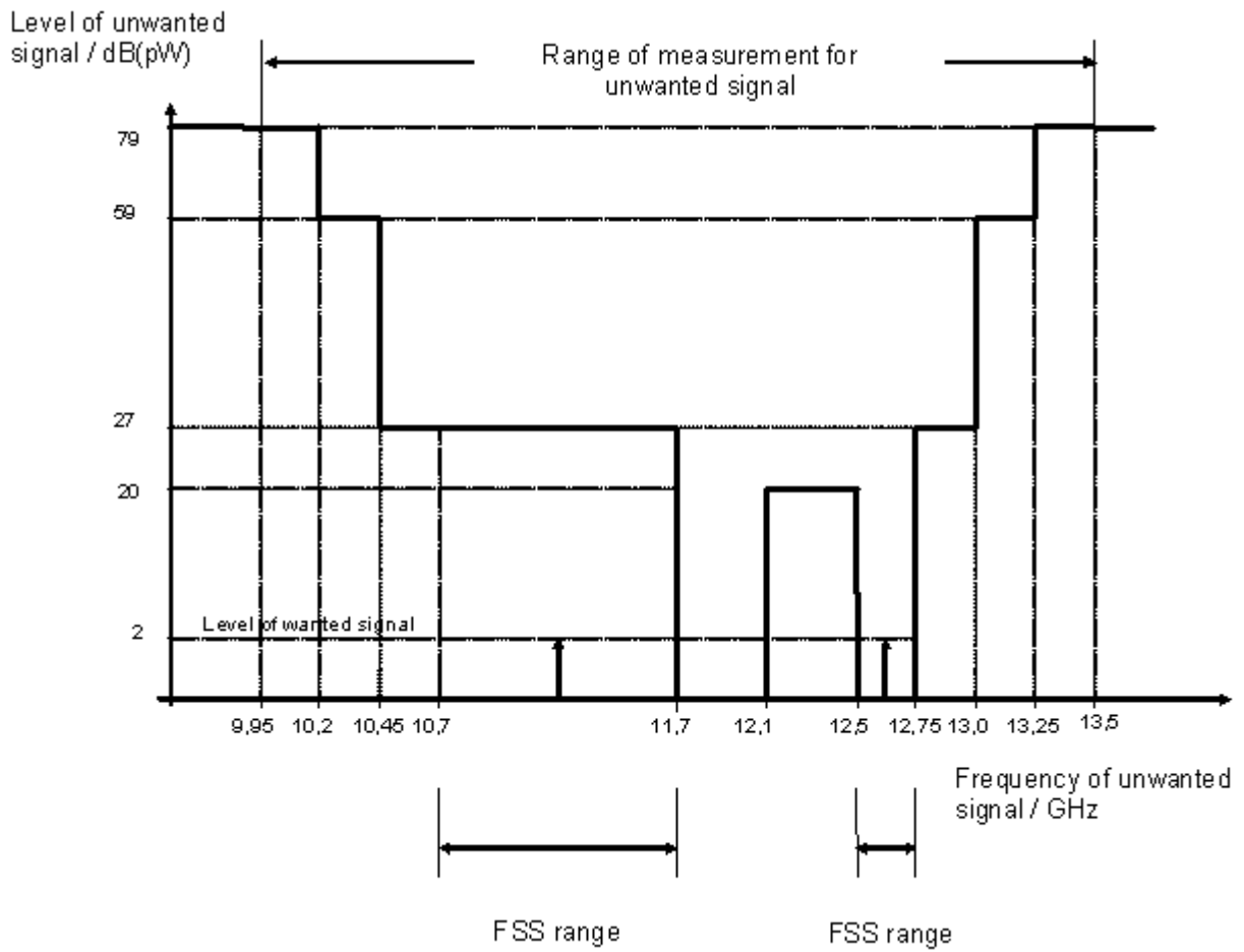
Figure 12 - Levels of wanted and unwanted signals for the internal immunity of FSS receiving outdoor units
