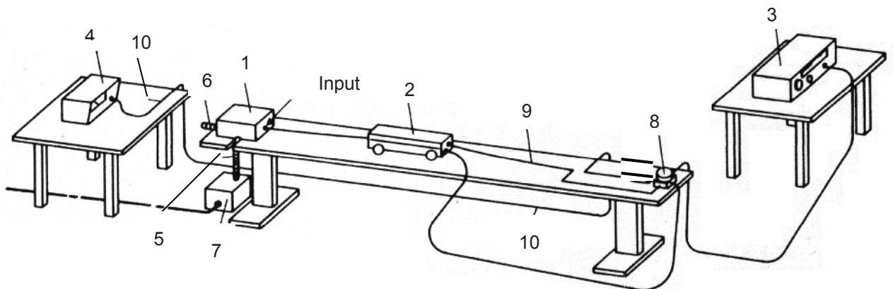
Figure 3 - Example of general measurement set-up
