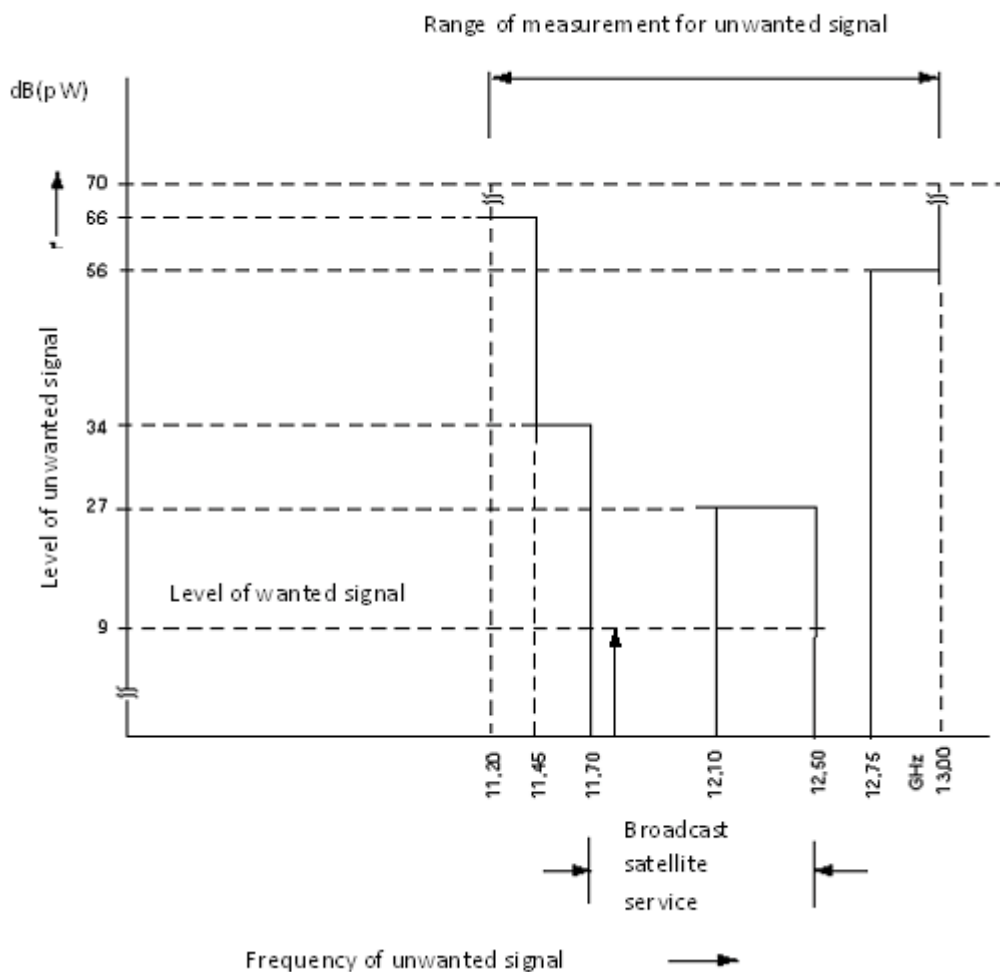
Figure 13 - Levels of wanted and unwanted signals for the internal immunity of BSS receiving outdoor units
