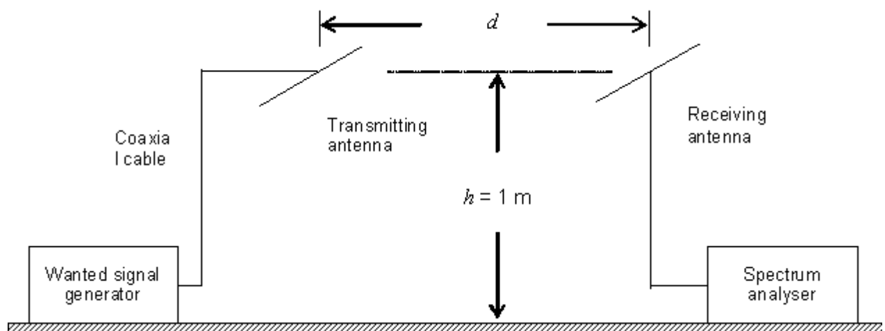
Figure 6 - Measurement set-up for the "substitution" radiation method – Second measurement step
