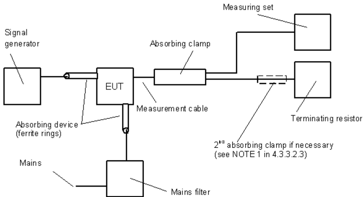
Figure 2 - Absorbing clamp method (30 MHz to 1 000 MHz)
