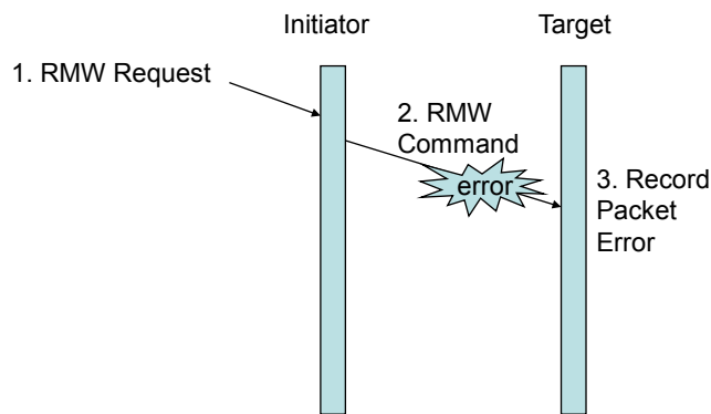
Figure 5-19: Read-Modify-Write Command Header Error
