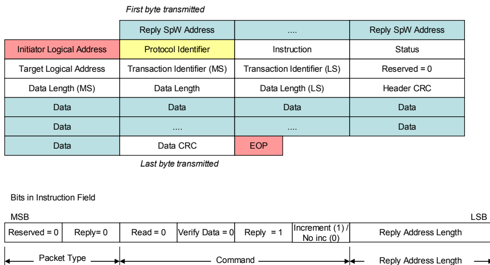
Figure 5-9: Read Reply format
