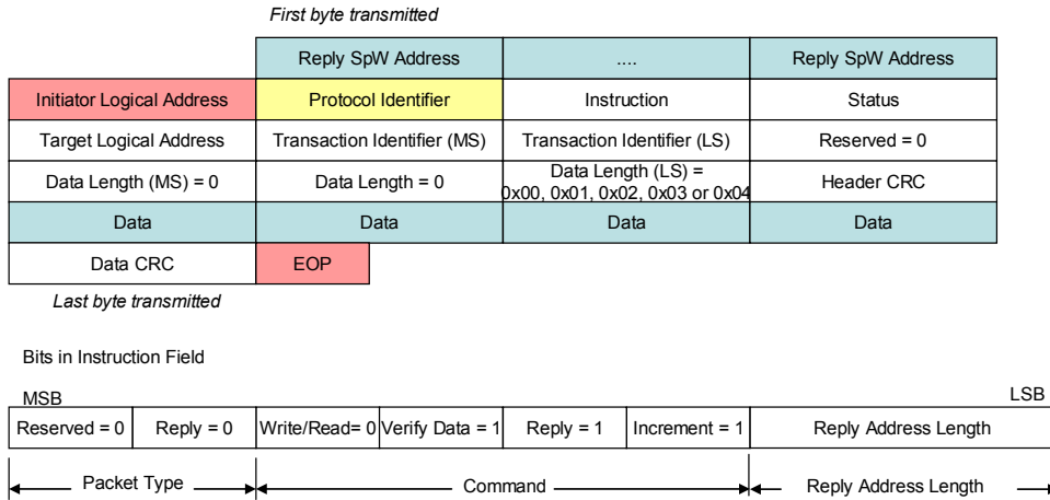
Figure 5-17: Read-Modify-Write Reply format
