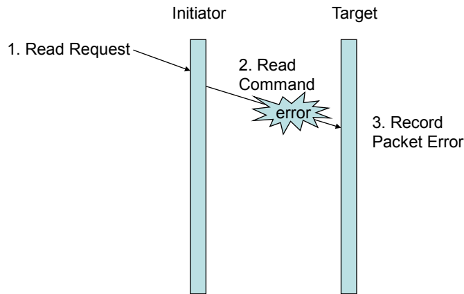
Figure 5-11: Read Command Header Error
