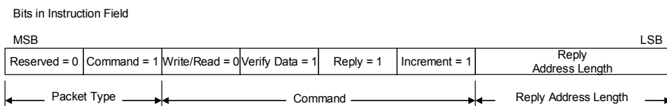
Figure 5-15: Read-Modify-Write Command format
