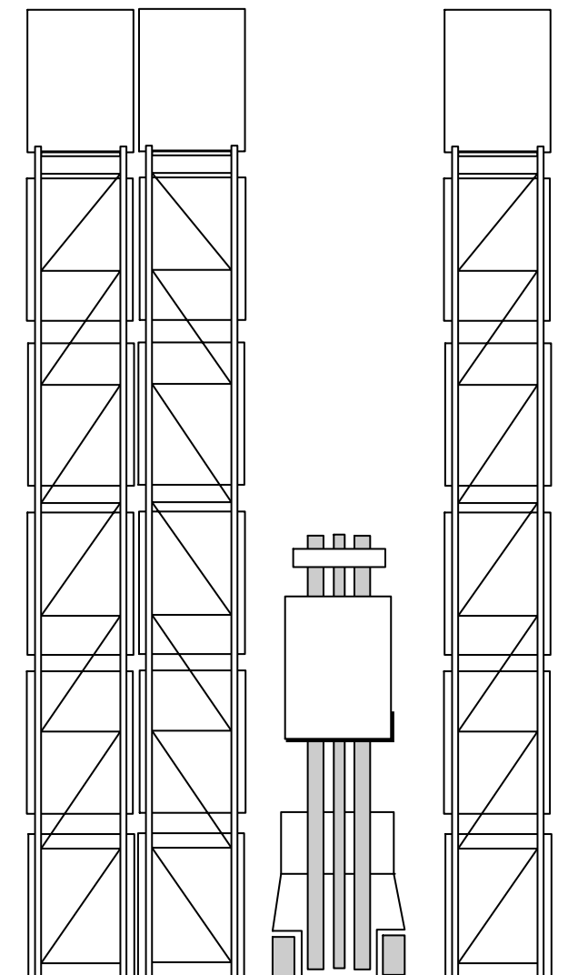
Figure 5 — Very narrow aisle racking
