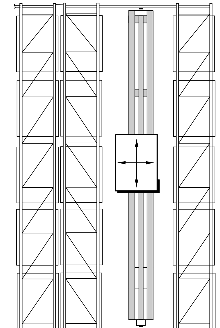
Figure 4 — Crane racking
