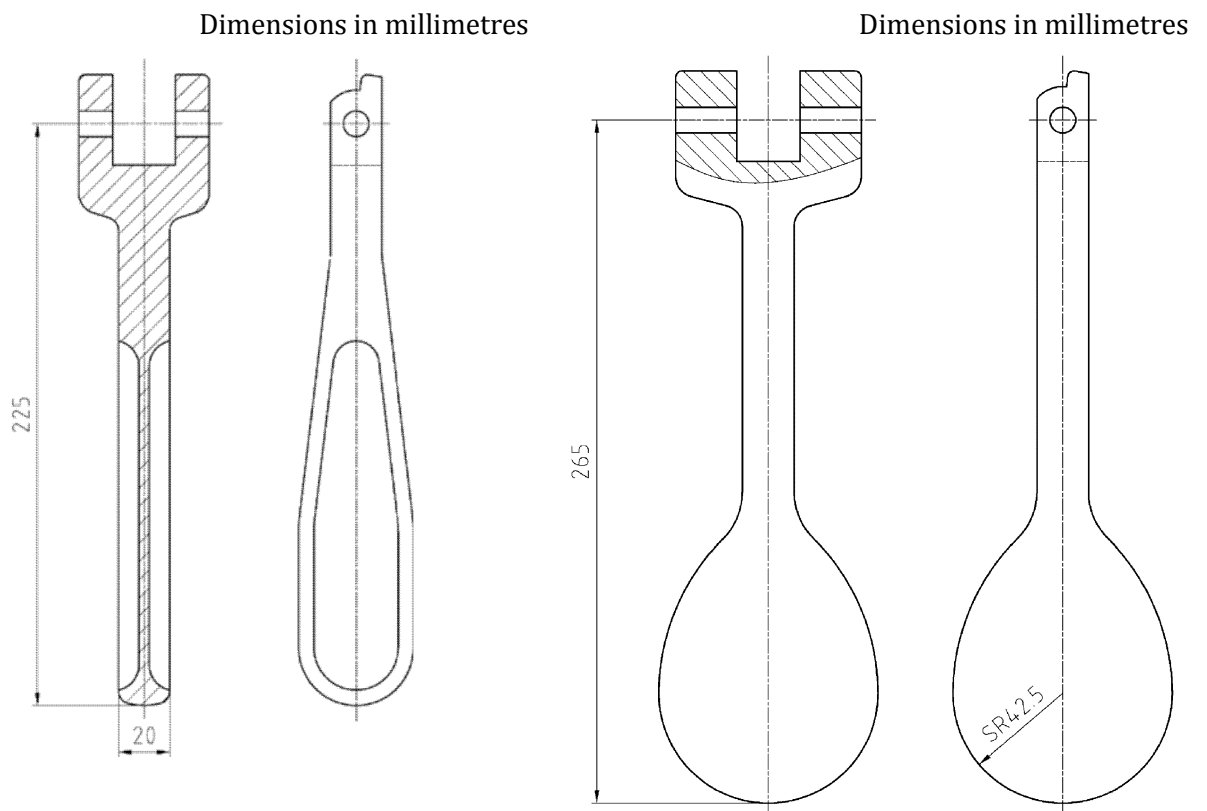
Figure D.2 — Hinged handle
