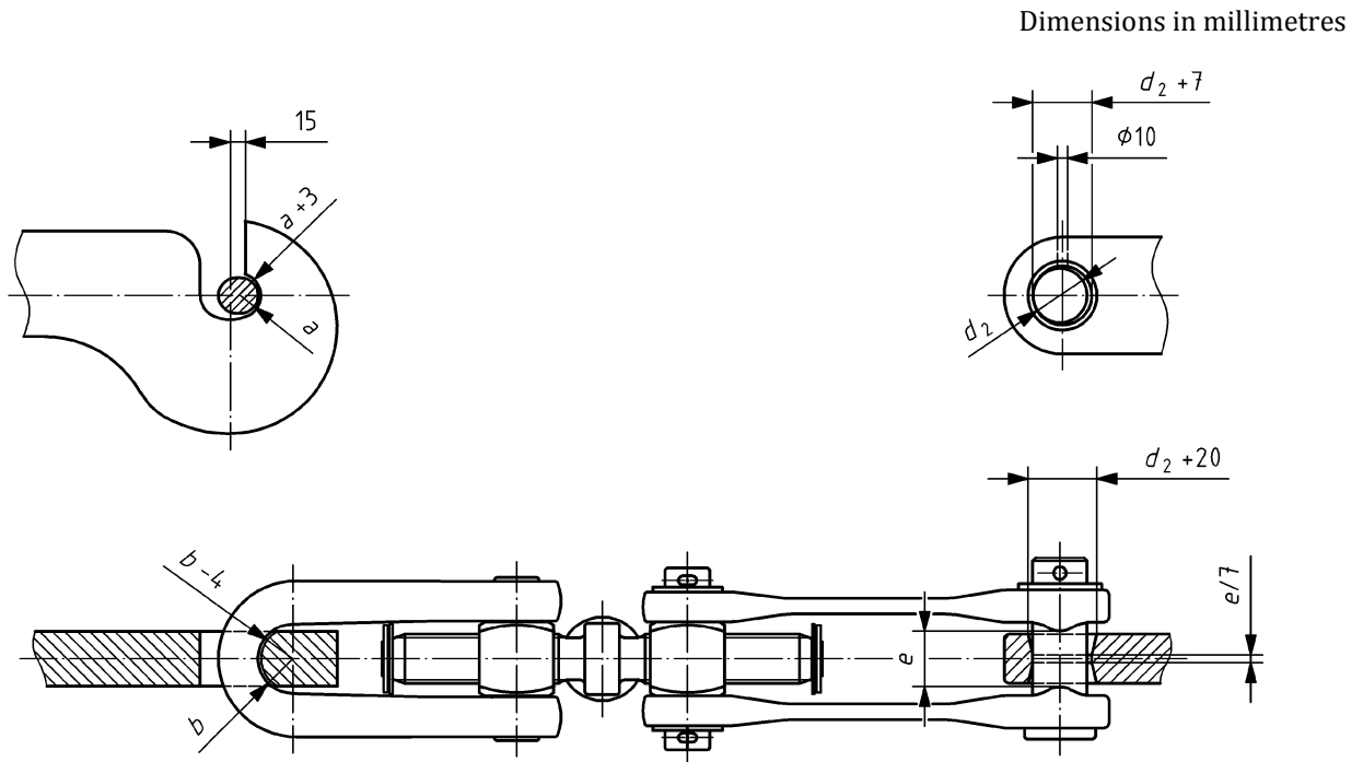
Figure F.2 — Test facility for the tensile test of the screw coupling
