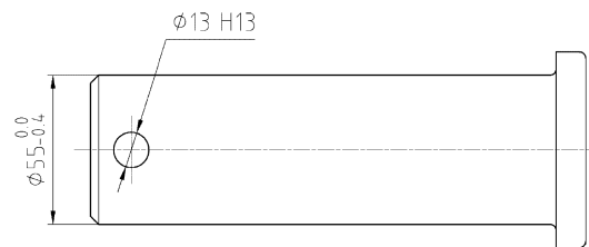
Figure D.1 — Coupling hook pin
