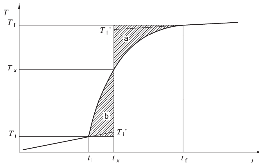
Figure B.1 — Dickinson extrapolation
