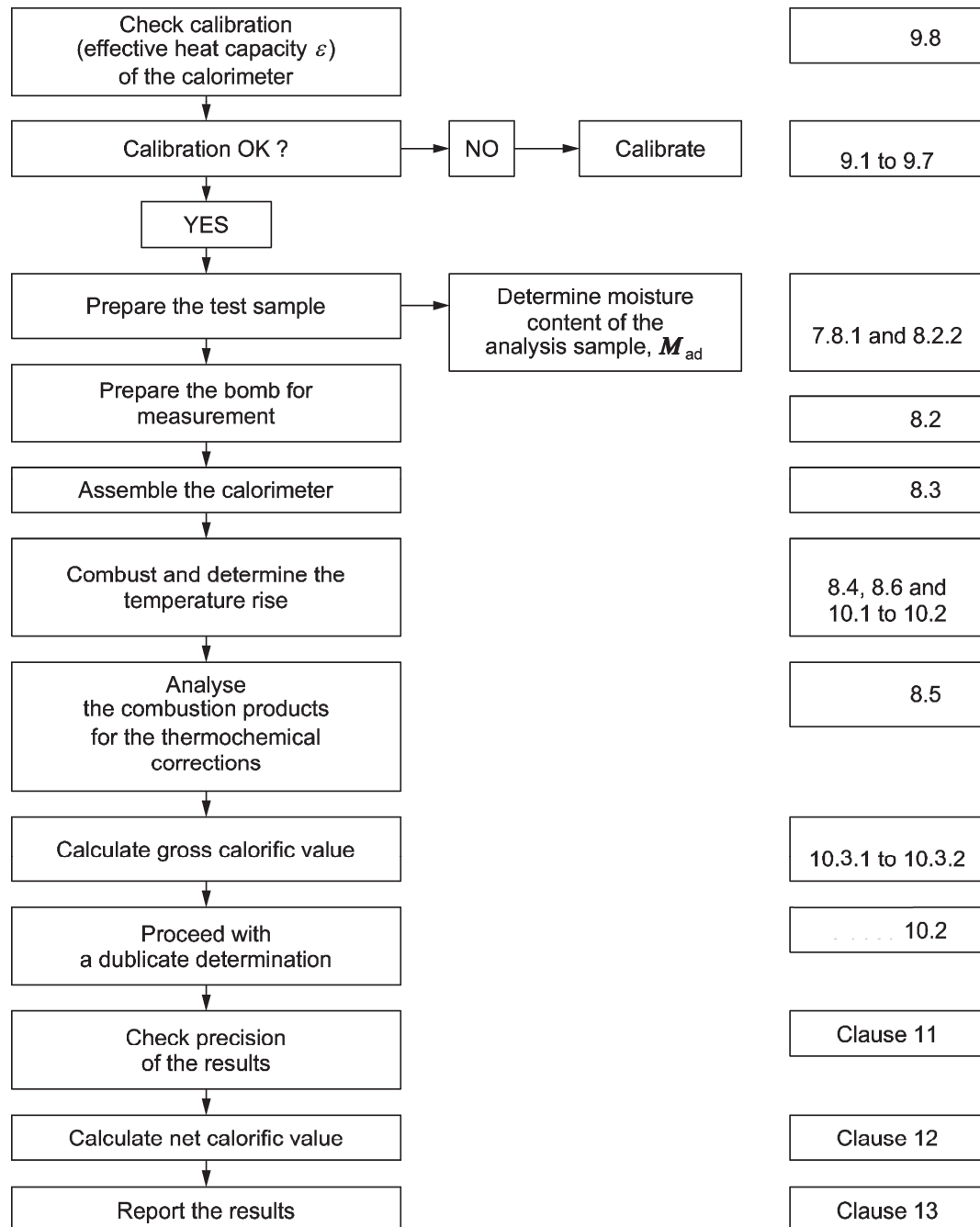
Figure H.1 — Flow chart for a routine calorific value determination
