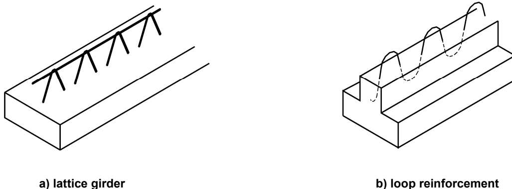
Figure 2 — Examples of connecting reinforcement
