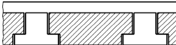
Figure B.4 — Floors with self-bearing beams
