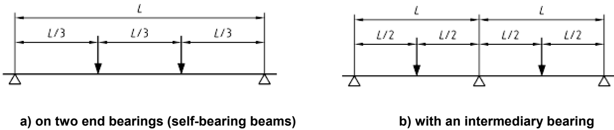
Figure H.2 — Loading arrangement for bending tests
