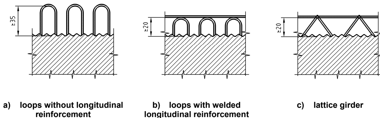
Figure 5 — Positioning of connecting reinforcement for good concreting and compaction
