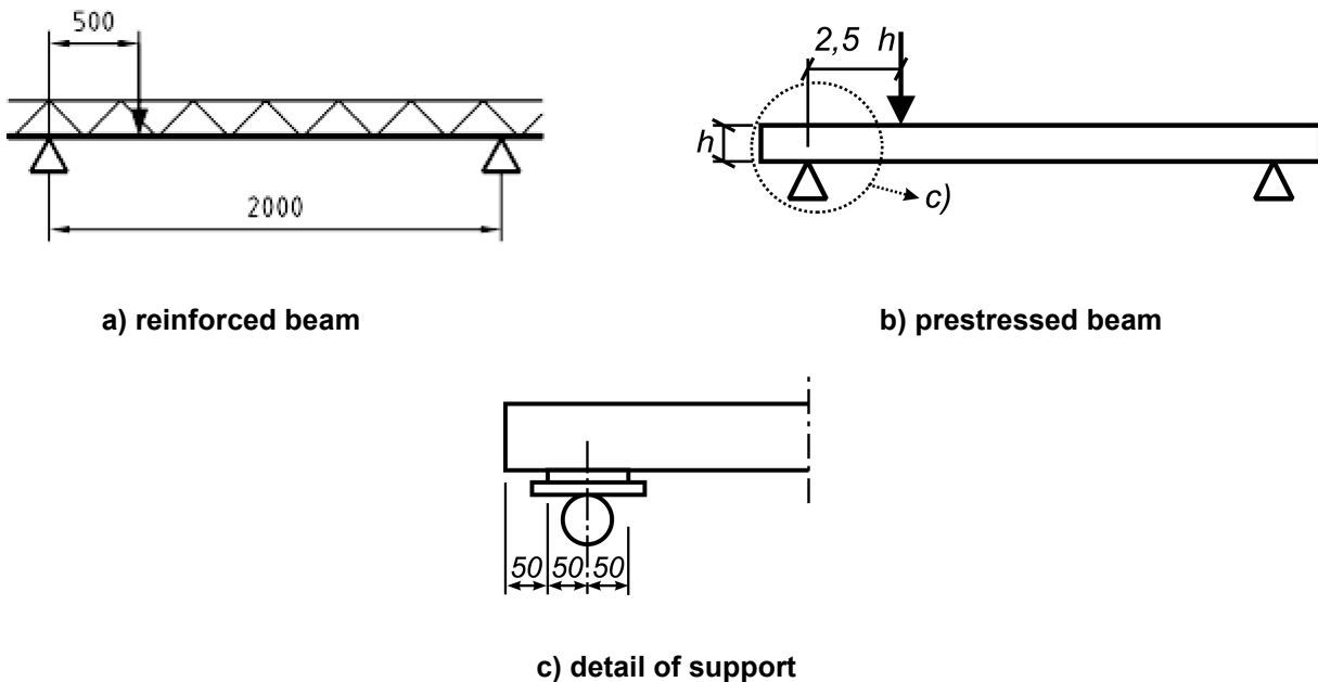
Figure H.3 — Loading arrangement for shear test
