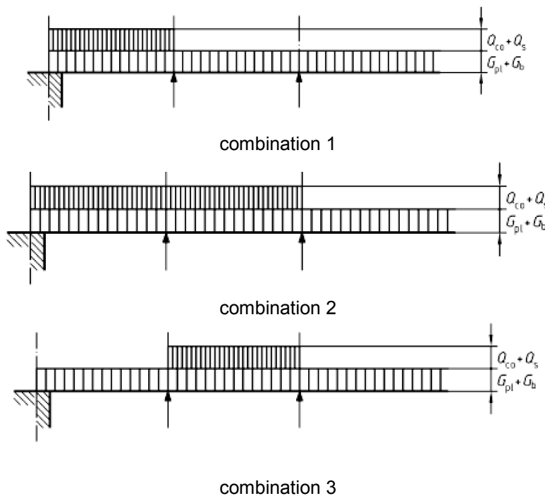
Figure H.1 — Static systems to be considered
