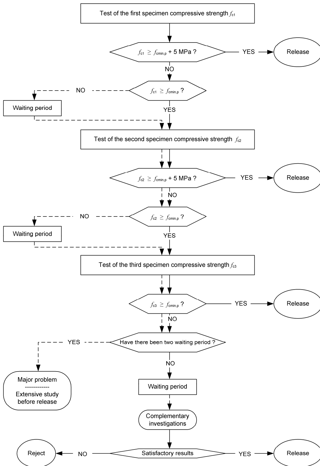
Figure J.1 — Tests procedure before release
