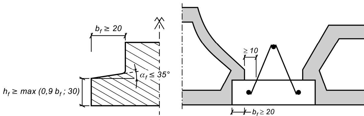
Figure 8 — Dimensions of toe rebate
