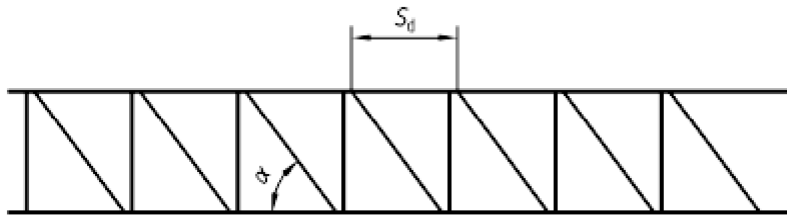
Figure E.11 — "PRAT" type lattice girder
