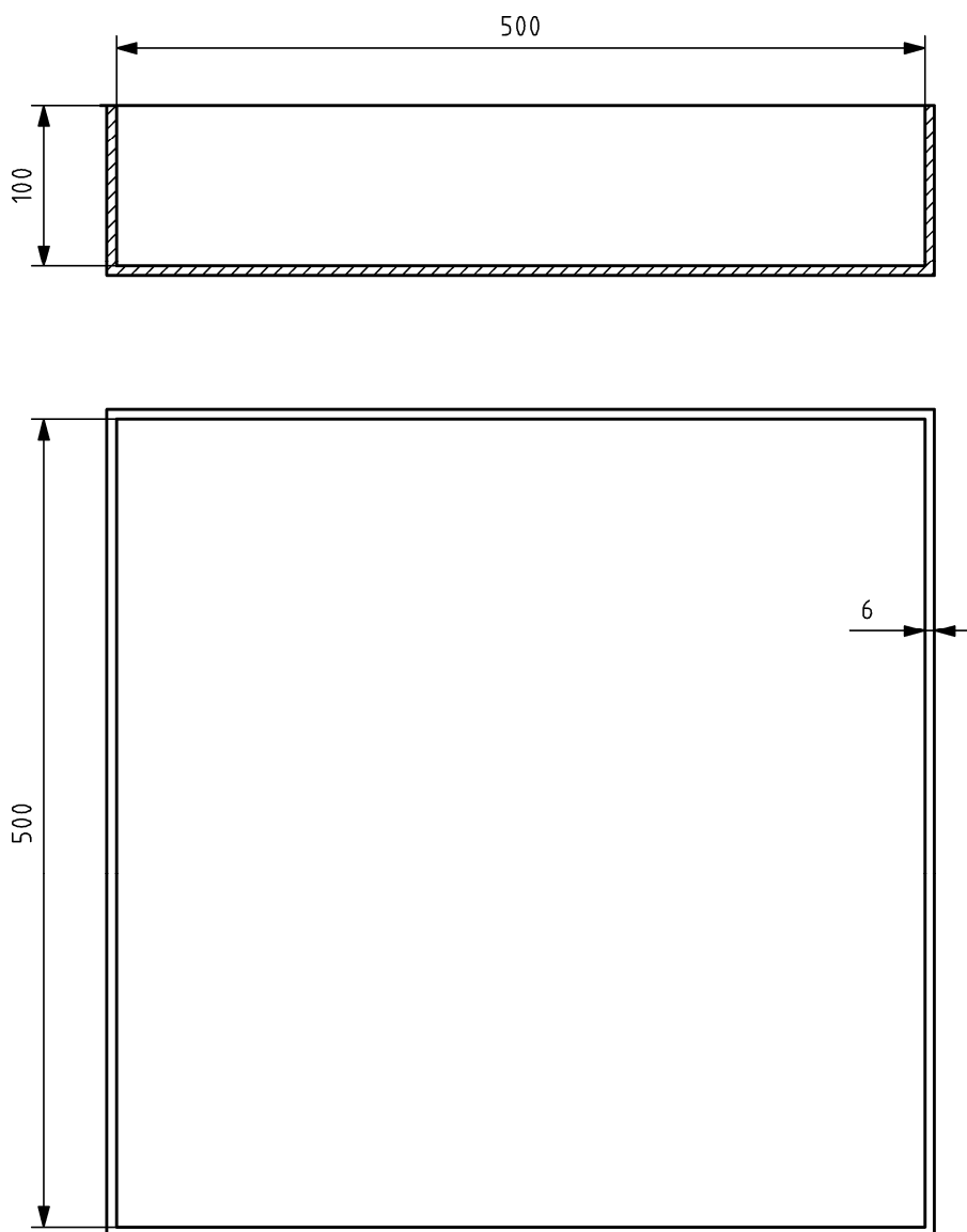
Figure C.7 — Pan geometry for wood crib and heptane pan fire test
