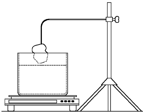
Figure C.1 — Example of an immersion apparatus
