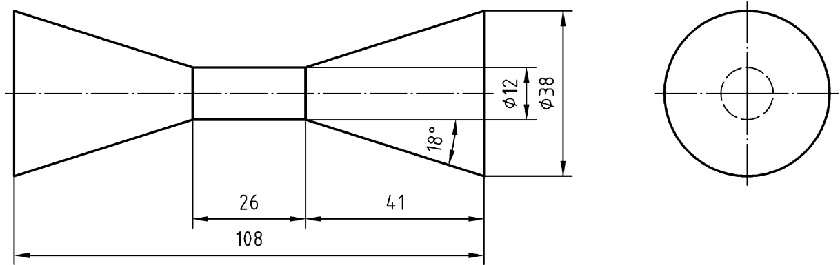
Figure C.1 — Dimensions of test specimens (mm)
