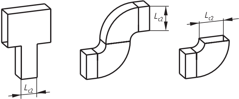
Figure 2 — Rectangular duct disturbances with the characteristic length L_{c1}
