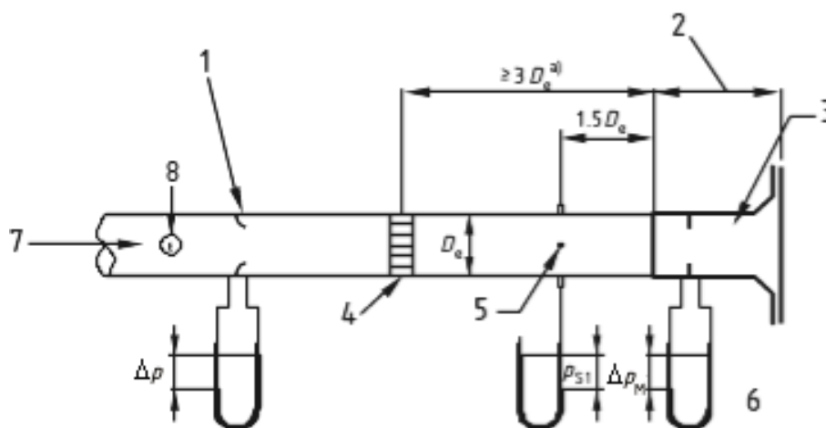
Figure 4 — Configurations A1 and A2 – Typical installation for IMS, undisturbed situation
