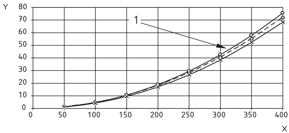
Figure 14 — Air flow rate as a function of output signal
