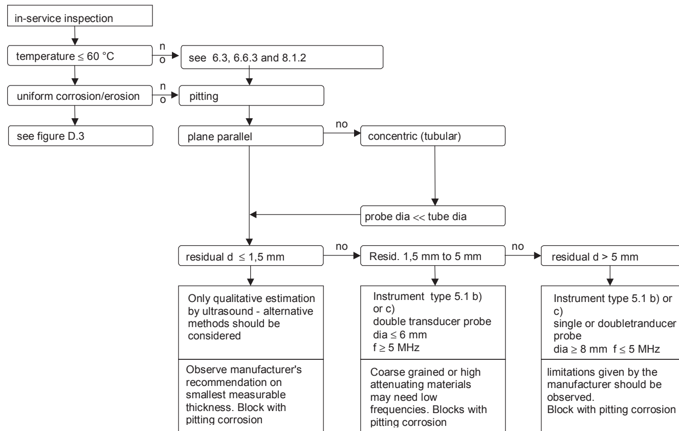
Figure D.4 — Flow chart for in-service inspection
