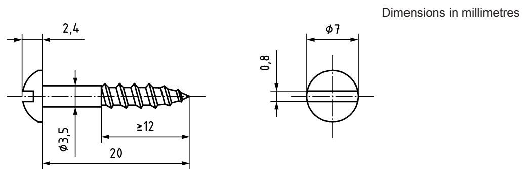
Figure H.2 — Fixing screw
