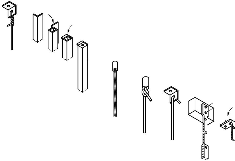
Figure 16 — Examples of different suspension components
