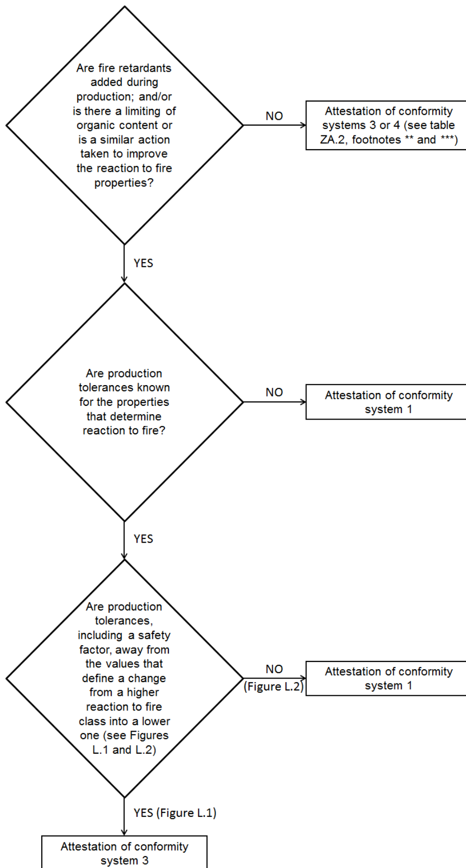
Figure L.3 - Flow chart demonstrating the decision making process
