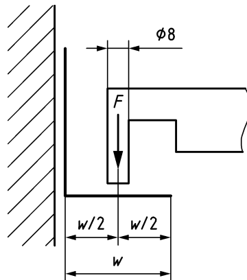
Figure H.4 — Load application
