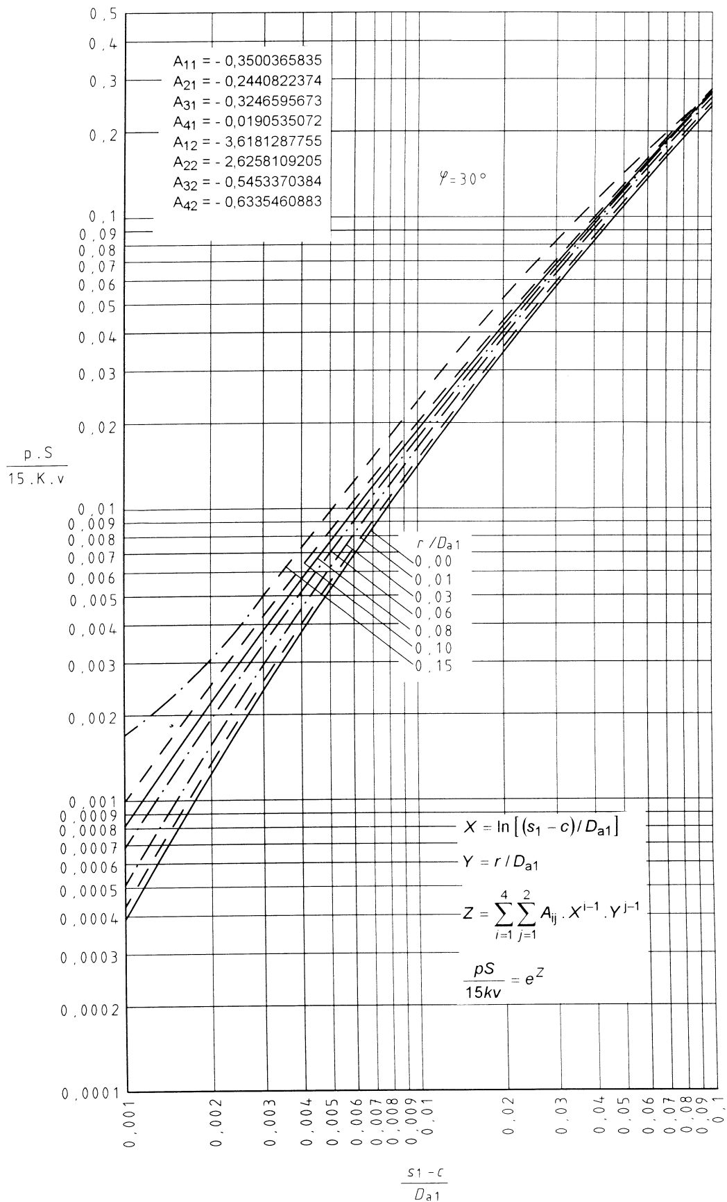
Figure 10 c) — Permissible value \frac{pS}{15Kv} for convergent cone with an opening angle \varphi = 30^\circ
