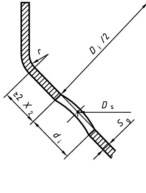
Figure 8 — Geometry of a cone opening
