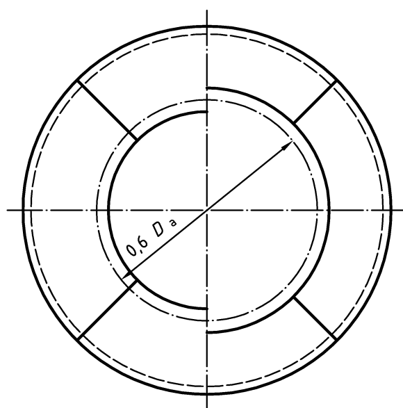
d) — Weld outside 0,6 D_a
