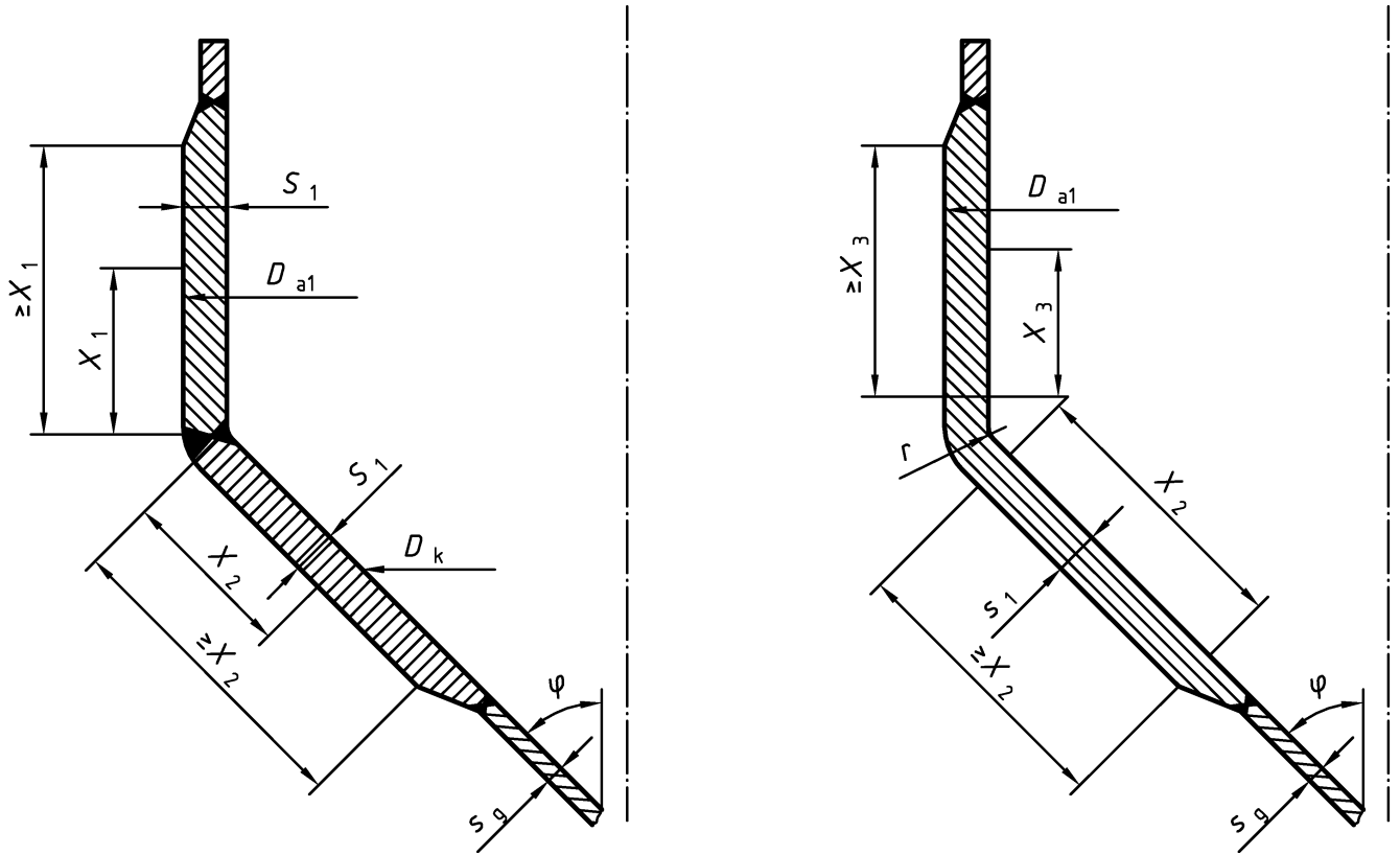
a) — Geometry of convergent conical shells
