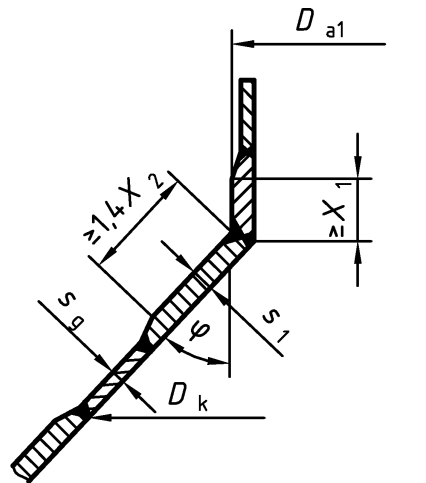
a) — Geometry of convergent conical shells
