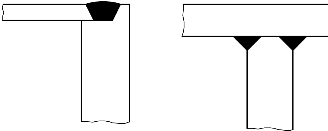
Figure F.4 — End plate closure (examples)
