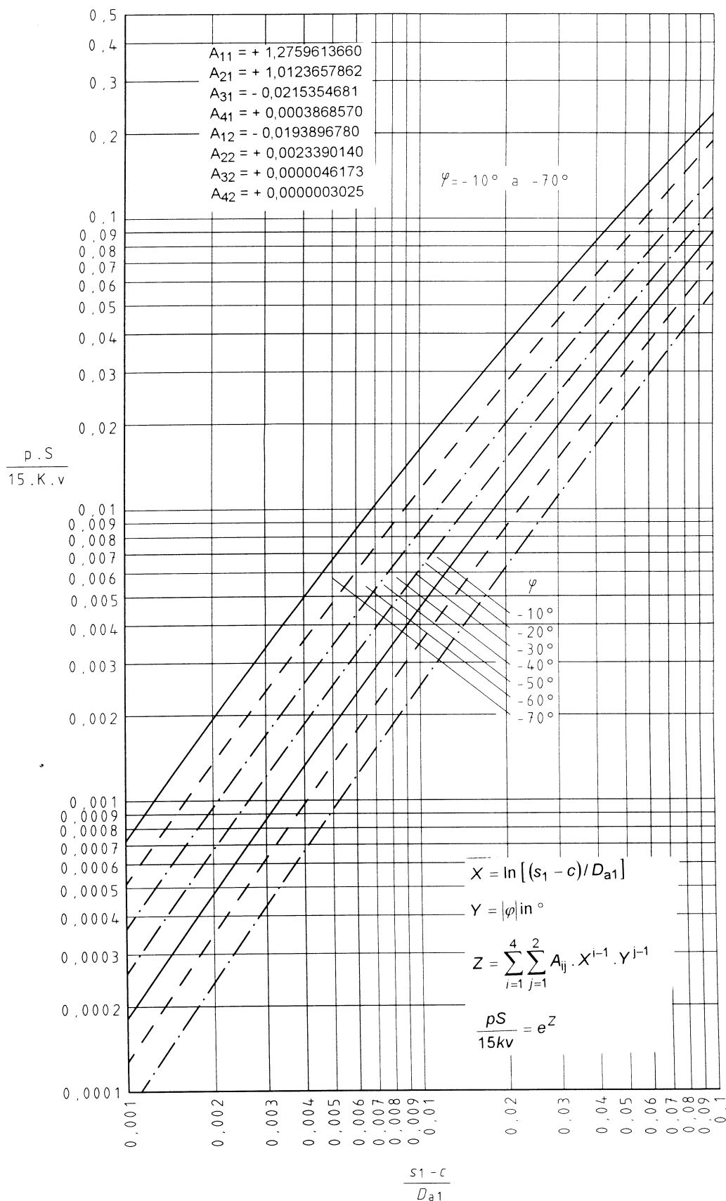
Figure 10 h) — Permissible value \frac{pS}{15Kv} for convergent cone (corner joint) with an opening angle \varphi = 10^\circ to 70^\circ
