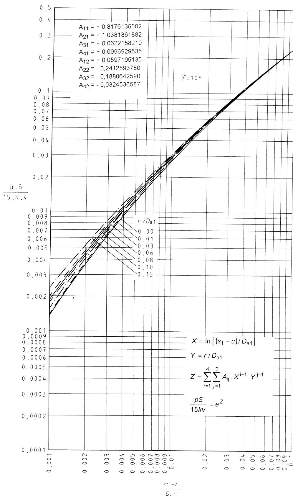
Figure 10 a) — Permissible value \frac{pS}{15Kv} for convergent cone with an opening angle \varphi = 10^\circ
