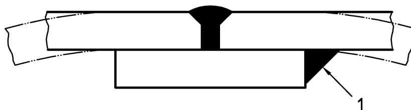
Figure F.2 — Intermediate end
