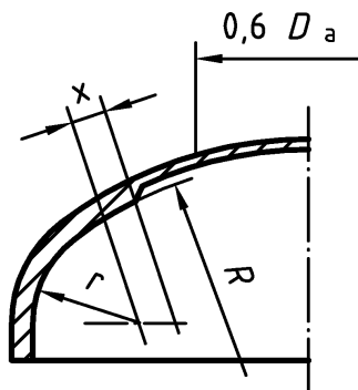
b) — Dished end with nozzle
