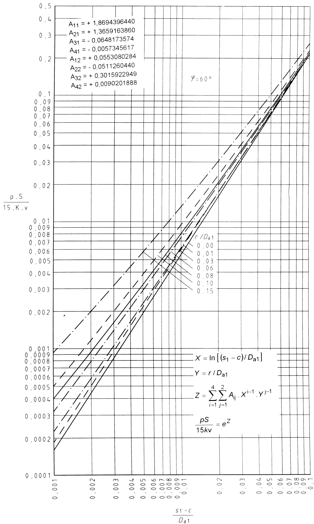
Figure 10 f) — Permissible value \frac{pS}{15KV} for convergent cone with an opening angle \varphi = 60^\circ
