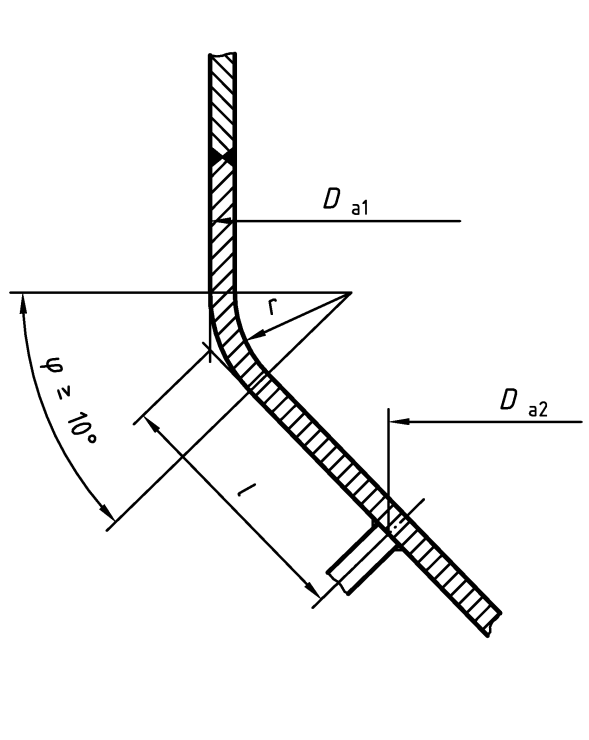
Figure 8 — Geometry of a cone opening
