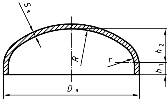
a) — Unpierced dished end
