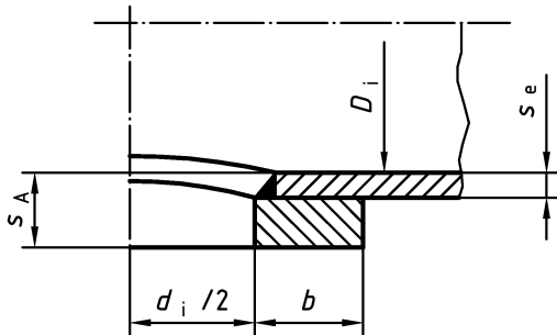
Figure 16 — Set-on reinforcement ring
