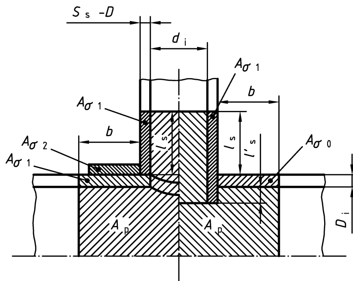
Figure 21 — Pad
