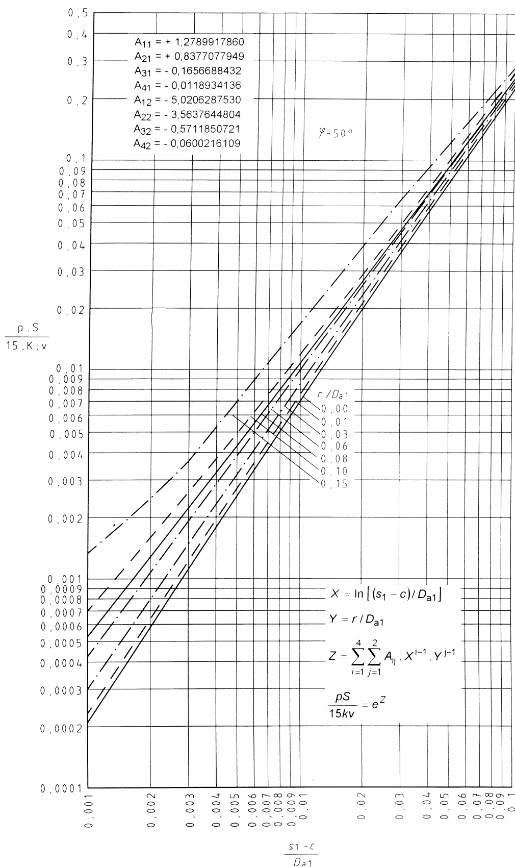
Figure 10 e) — Permissible value \frac{pS}{15Kv} for convergent cone with an opening angle \varphi = 50^\circ
