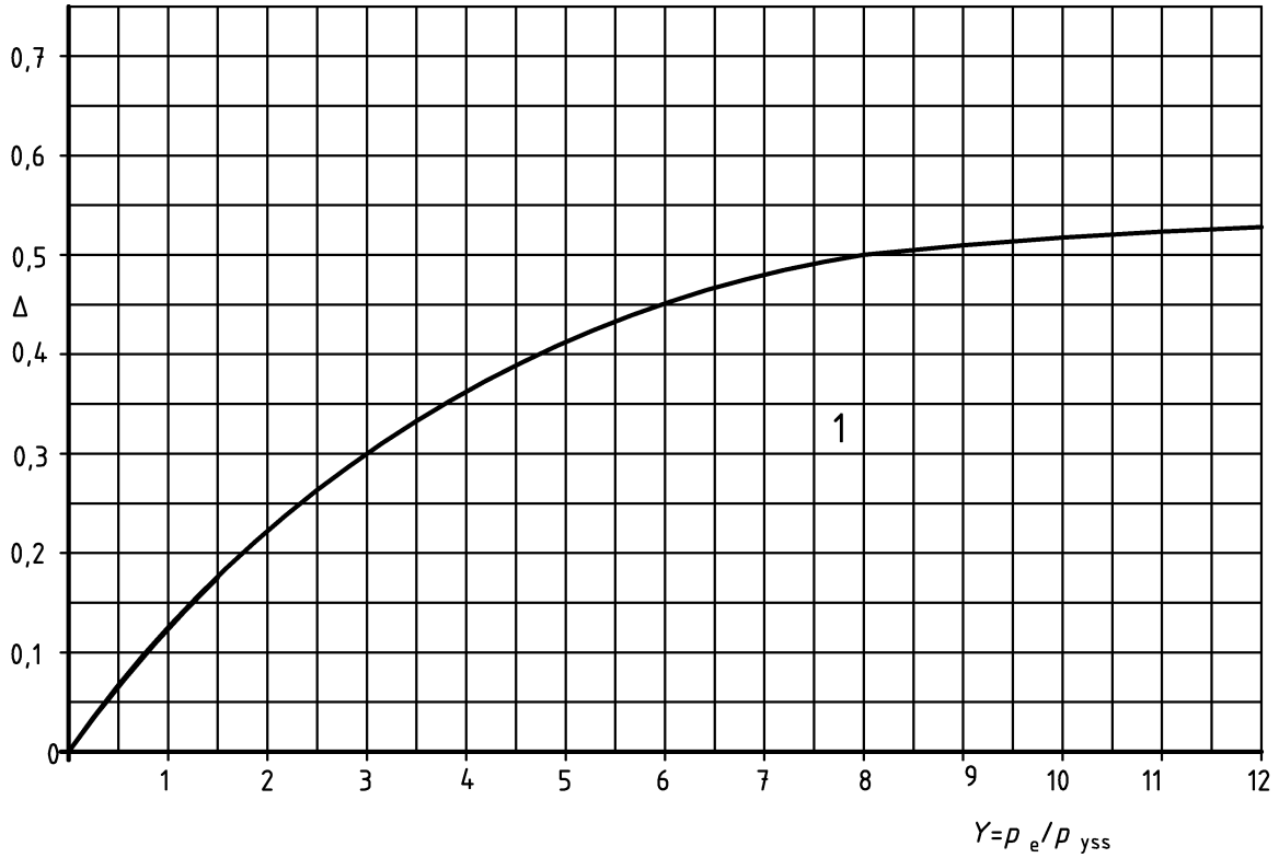
Figure A.2 — For vessels subject to external pressure
