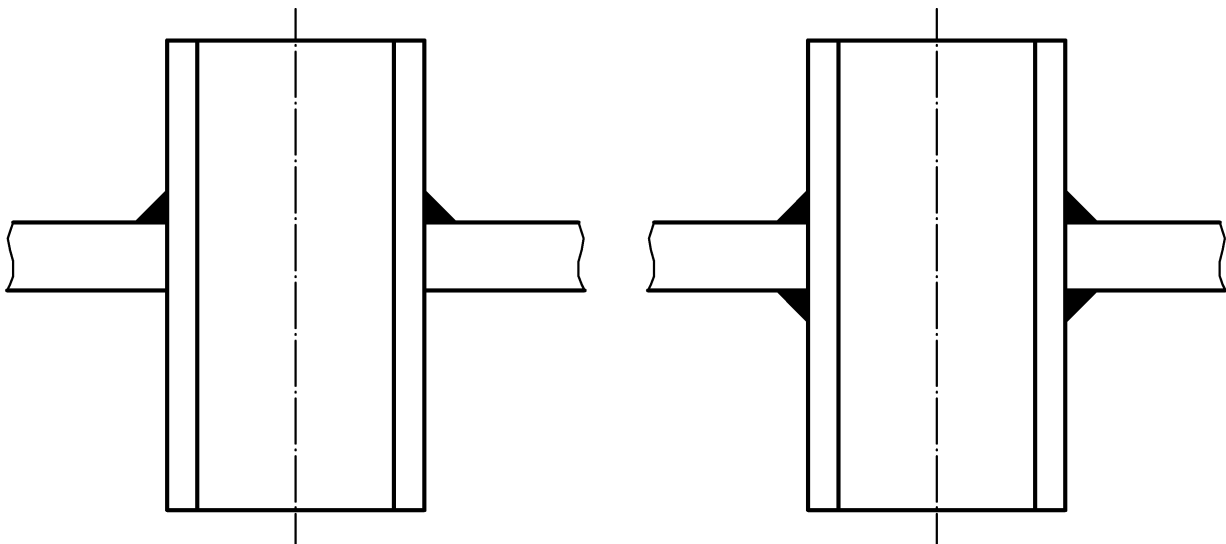
Figure F.4 — End plate closure (examples)
