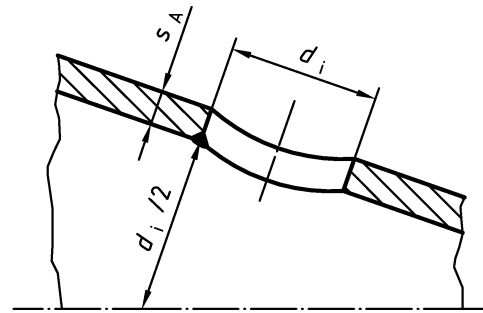
Figure 15 — Increased thickness of a conical shell
