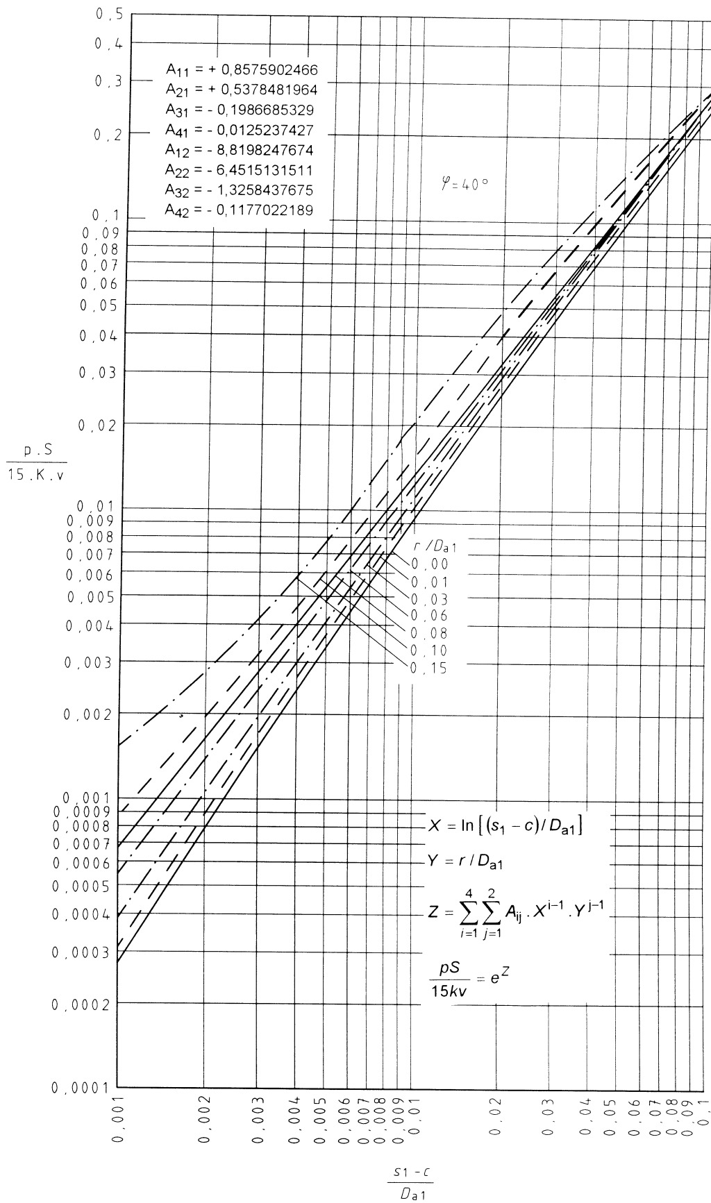
Figure 10 d) — Permissible value \frac{pS}{15Kv} for convergent cone with an opening angle \varphi = 40^\circ
