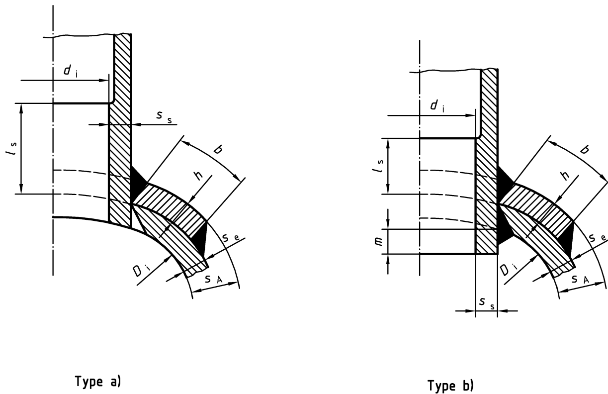
Figure 21 — Pad
