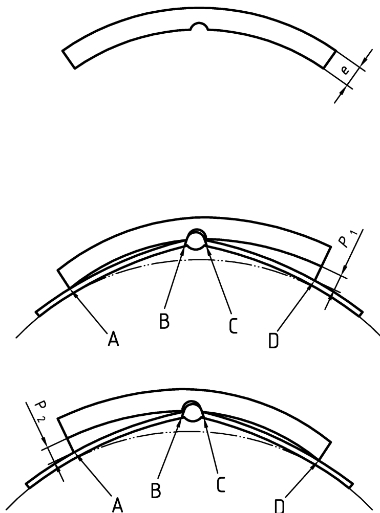
Figure 28 — Gauge details
