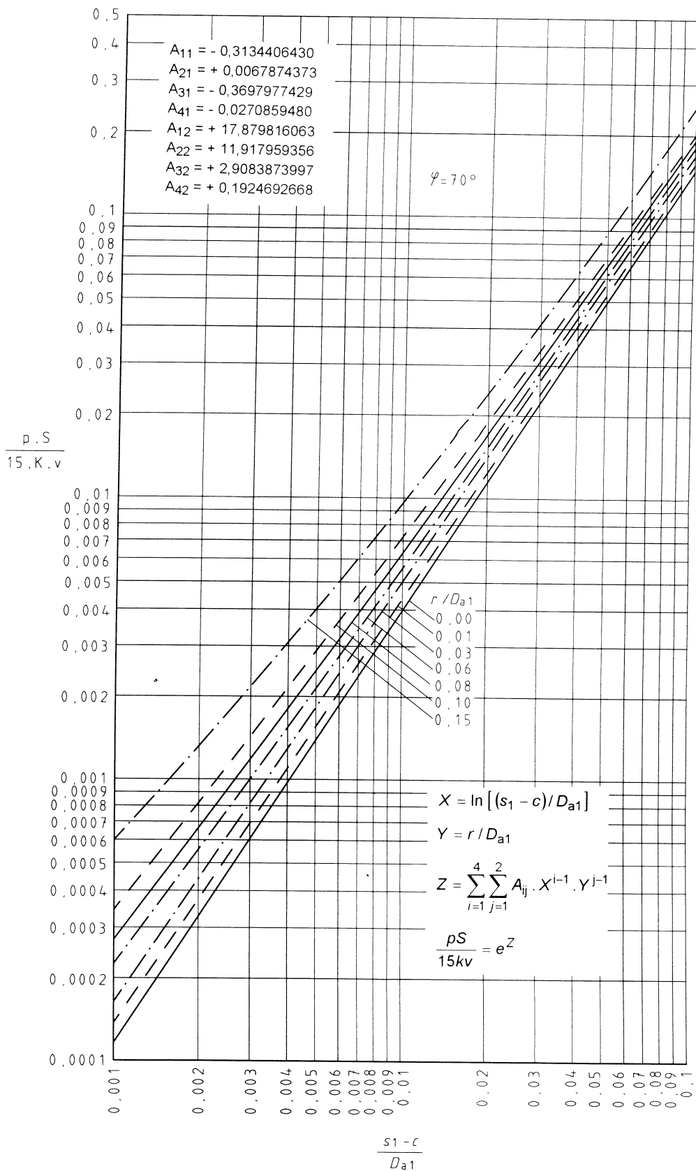
Figure 10 g) — Permissible value \frac{pS}{15KV} for convergent cone with an opening angle \varphi = 70^\circ
