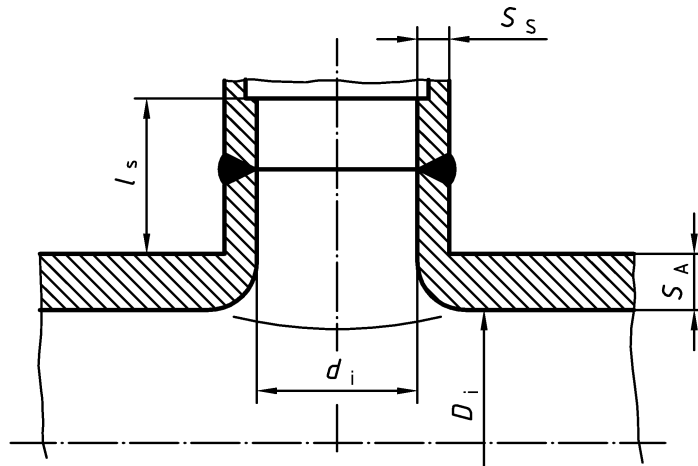
Figure 19 — Nozzle reinforcement
