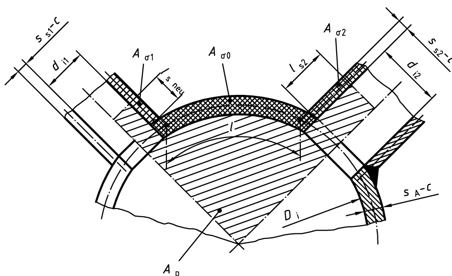
Figure 25 — Openings between longitudinal and circumferential direction
