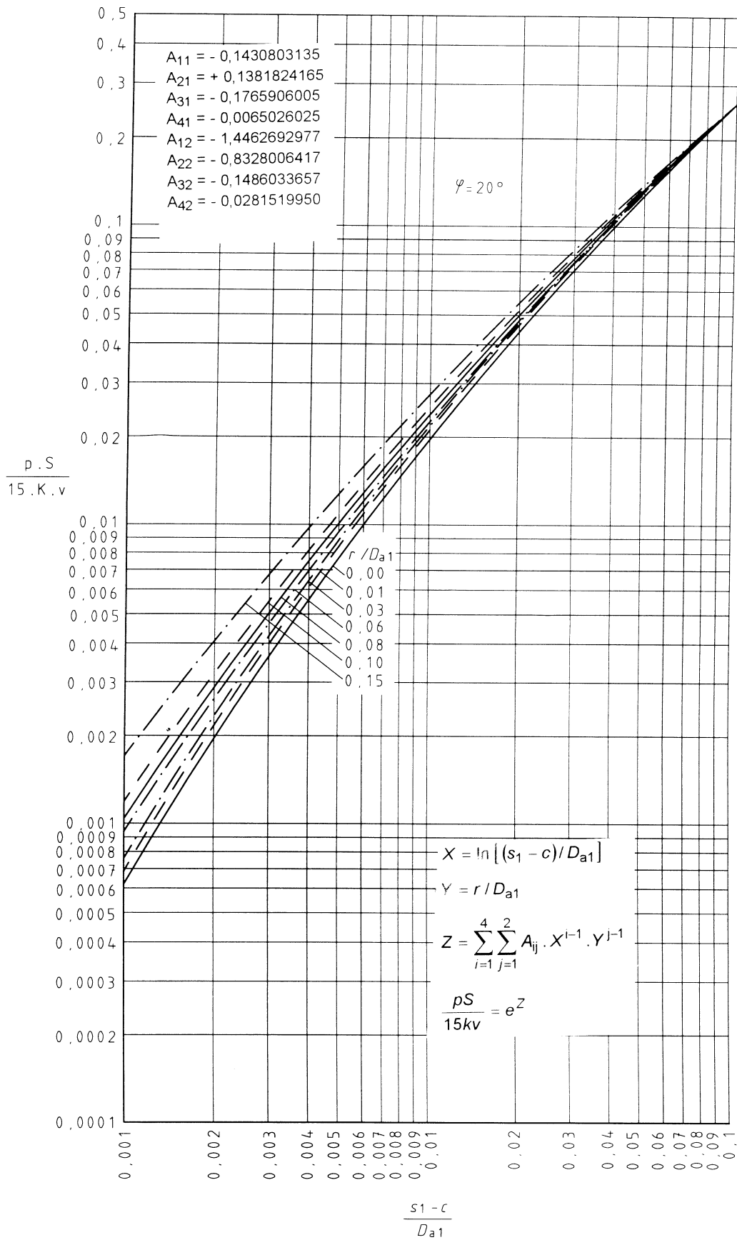
Figure 10 b) — Permissible value \frac{pS}{15Kv} for convergent cone with an opening angle \varphi = 20^\circ
