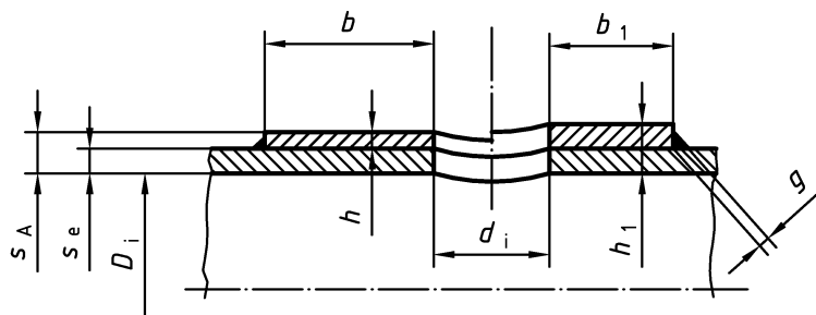
Figure 18 — Pad reinforcement
