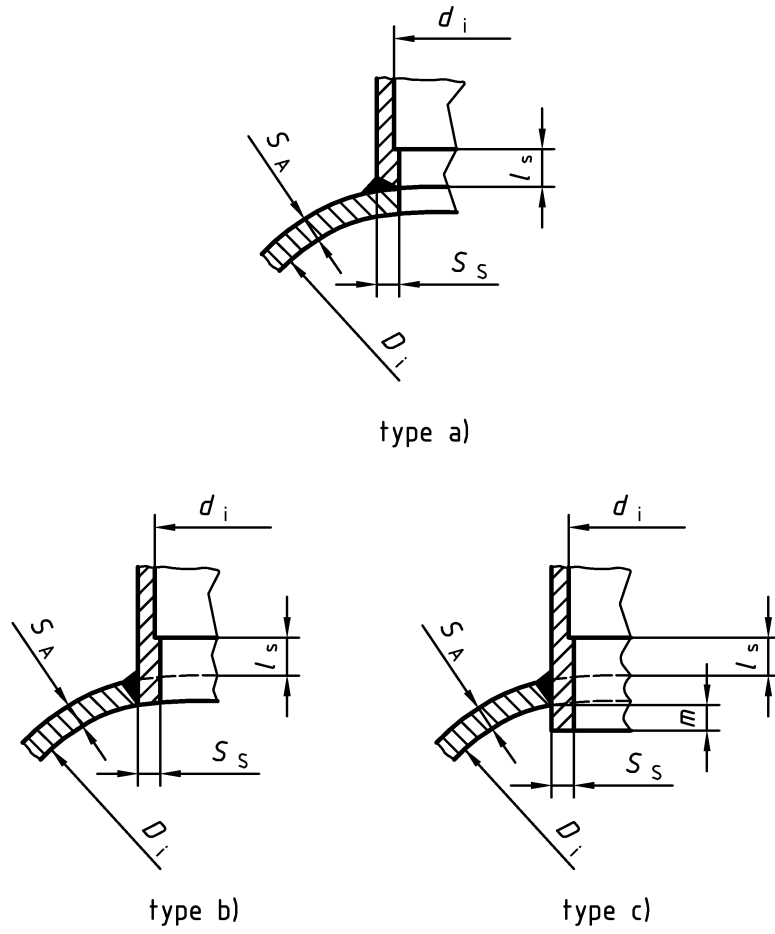
Figure 19 — Nozzle reinforcement
