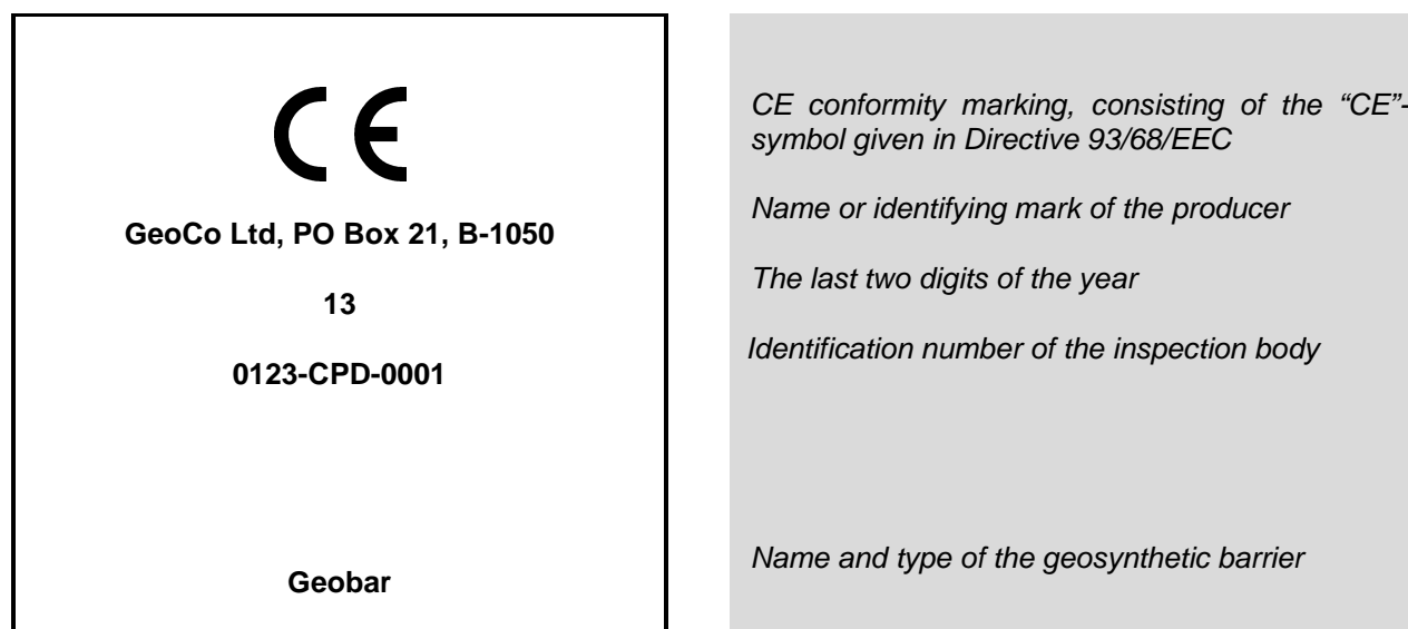
Figure ZA.1 — Example of CE marking on the packaging of a Geosynthetic Barrier
