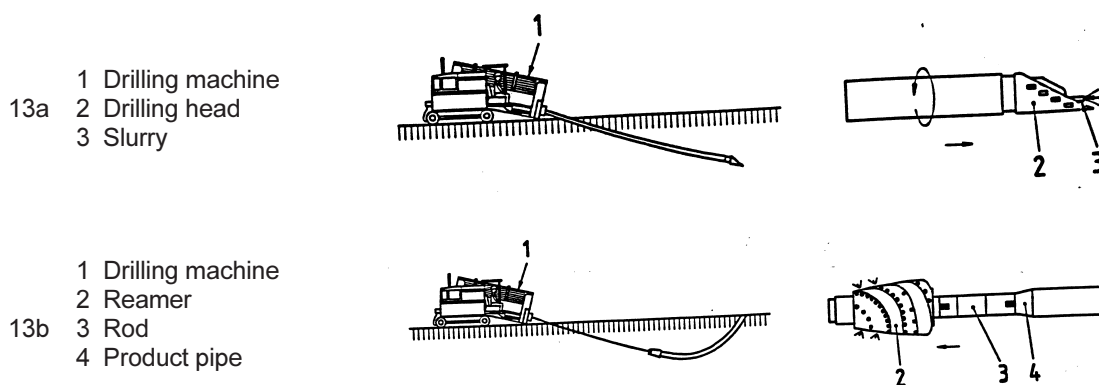
Figure 13: Example of directional drilling
