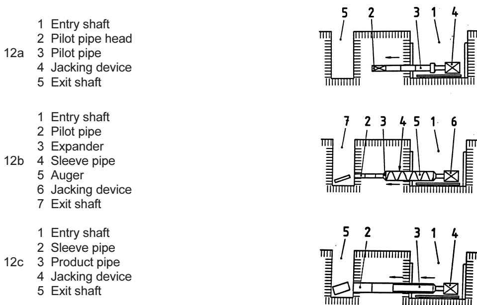
Figure 12: Example of pilot jacking with pipe bore
