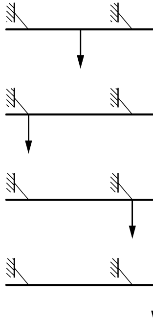
Figure F.3 — Placement of test loads for collective top protection systems
