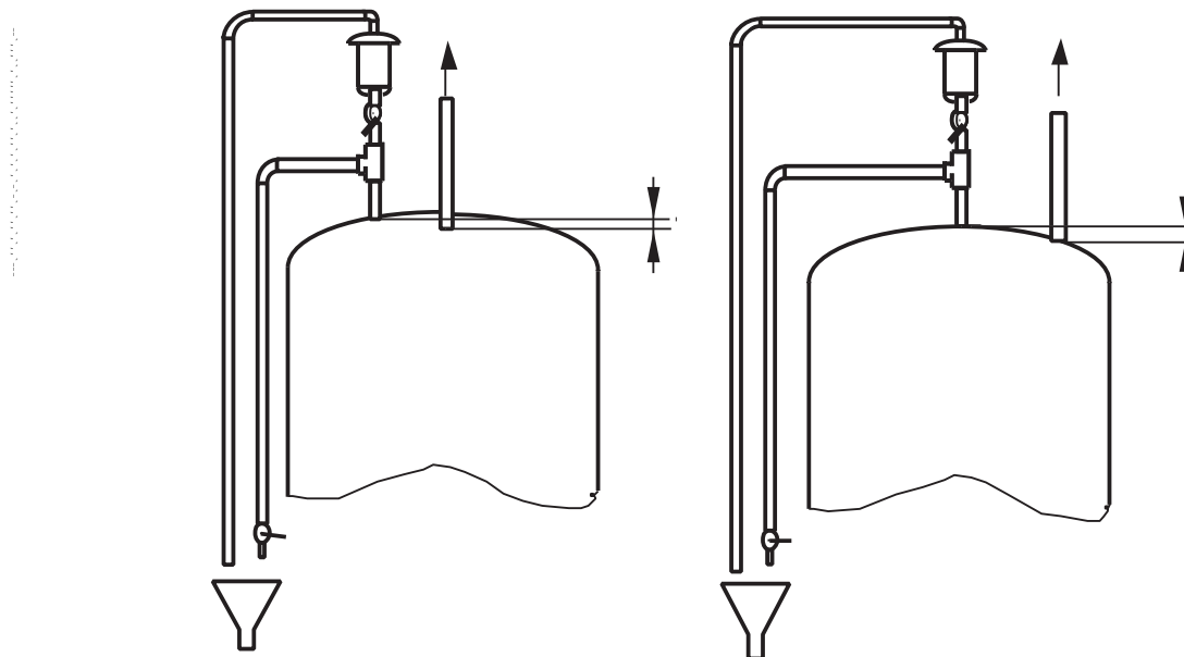
Figure 3 — Examples of locations of water and venting outlets
