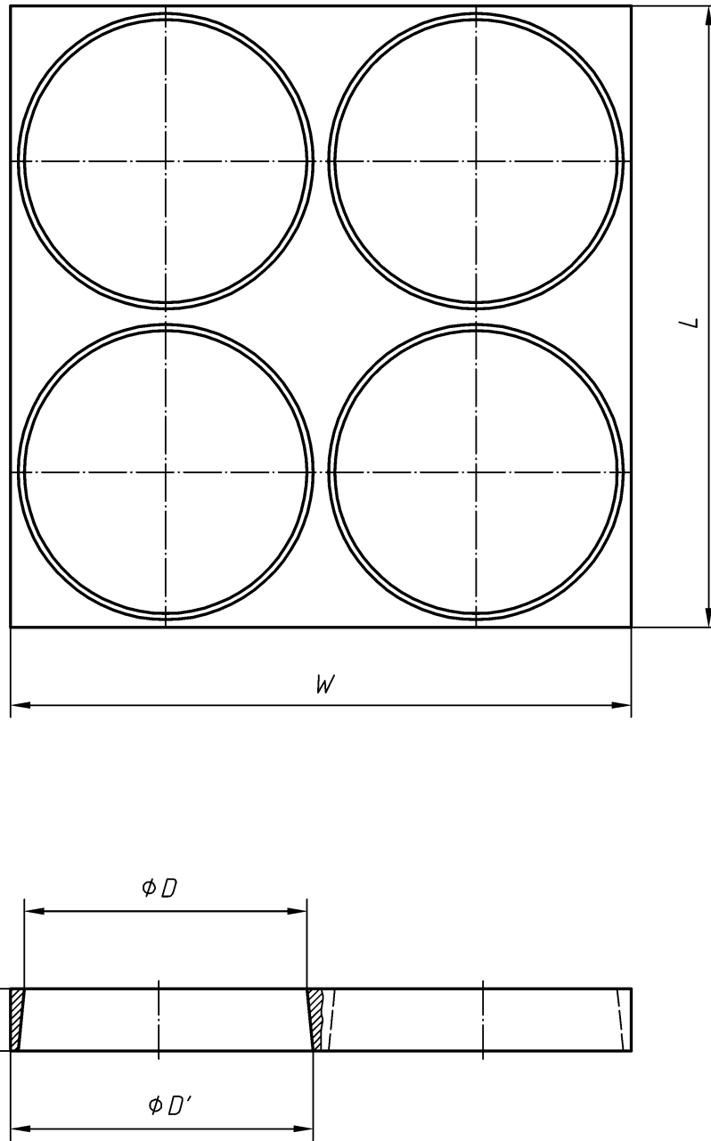
Figure 1 — Metal square-shaped moulds, upper view, side view
