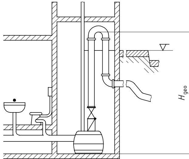
Figure 8 — Static head
