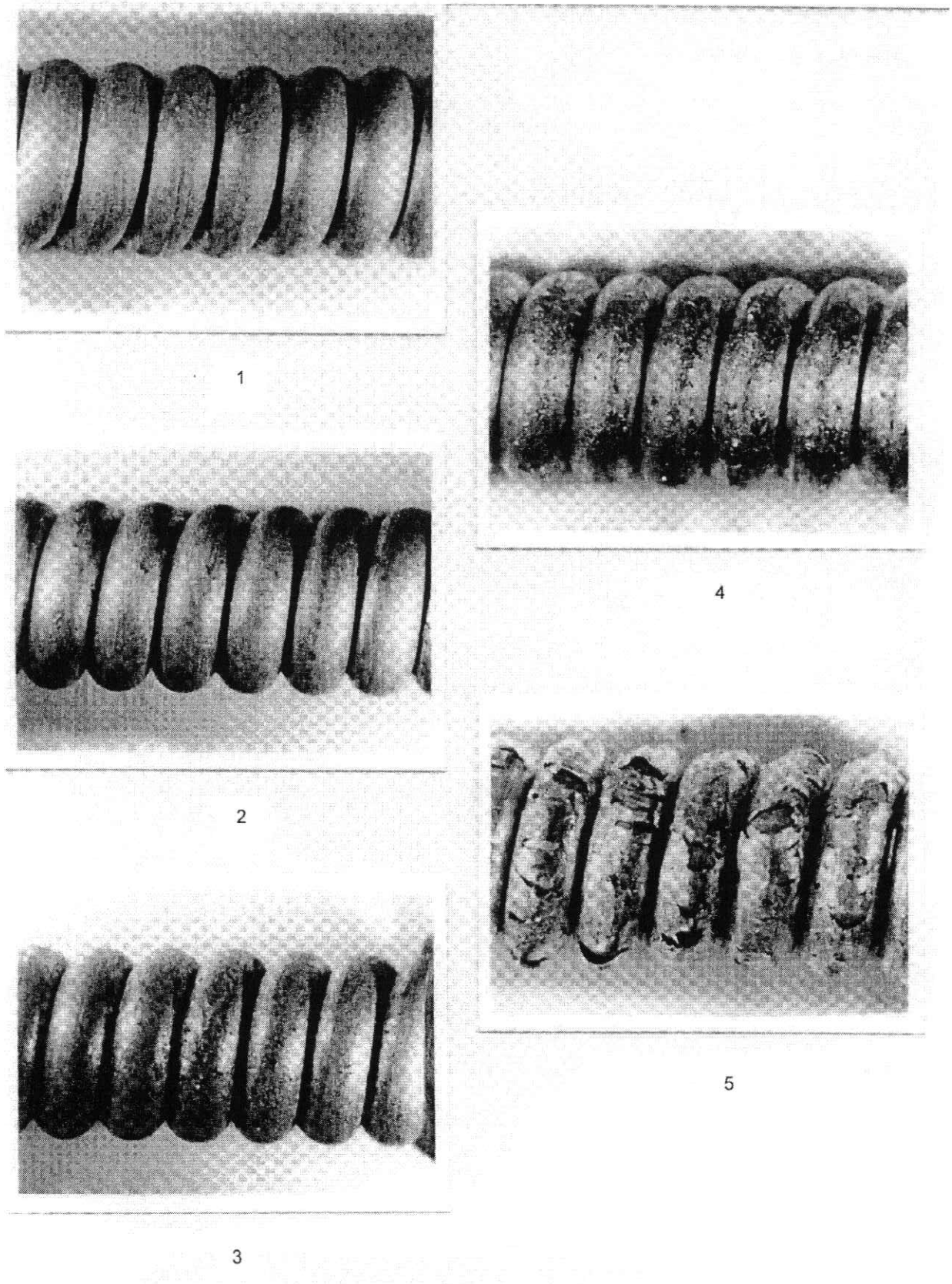
Figure 1 — Assessment of the adherence of the coating
