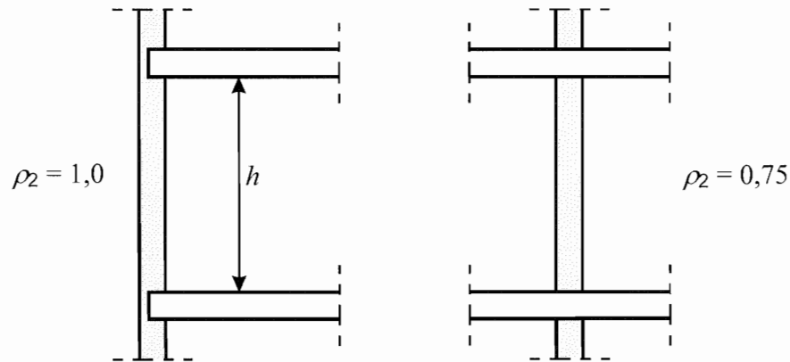
Figure 4.3 — Rotational restraint provided by floors or roof
