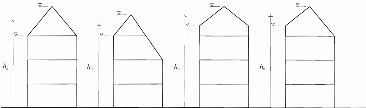
Figure 4.1 — Determination of average height
