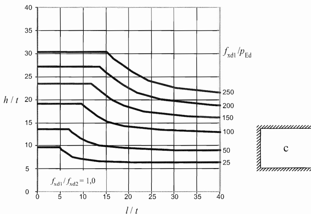
Figure C.7 – Thickness and size limitation of non-bearing walls with lateral loading. Wall type c – f_{xd1}/f_{xd2} = 1,0
