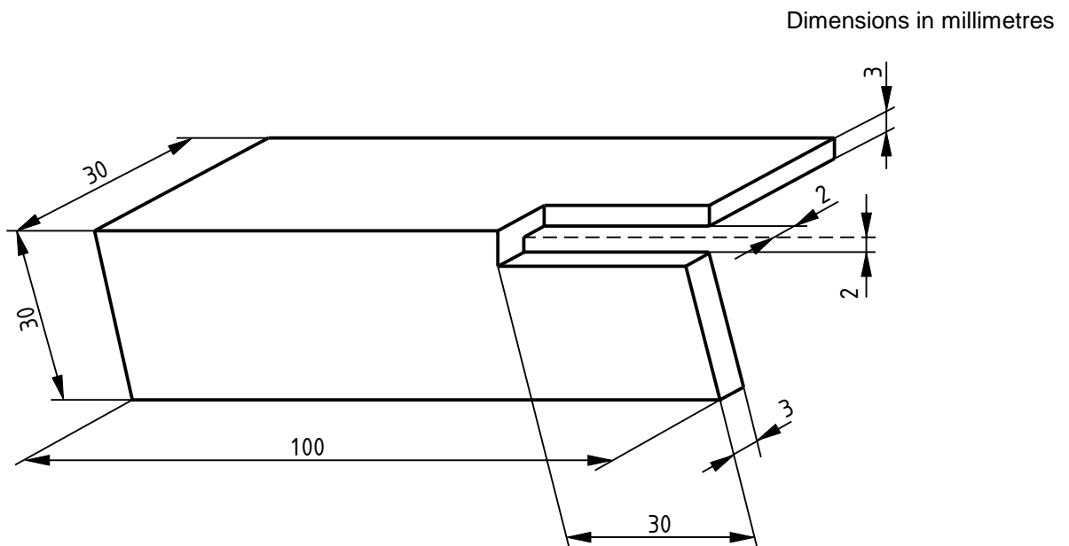
Figure 5 — Breakage defect sizer
