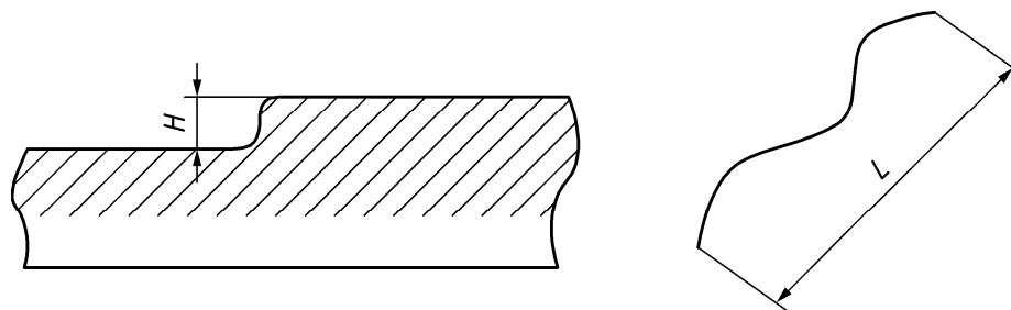
Figure 2 — Step irregularities
