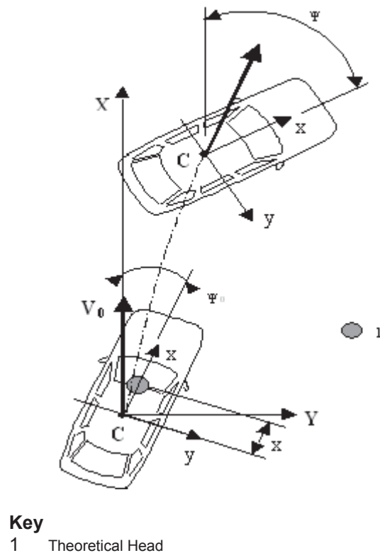
Figure 7 — Vehicle and ground reference frames
