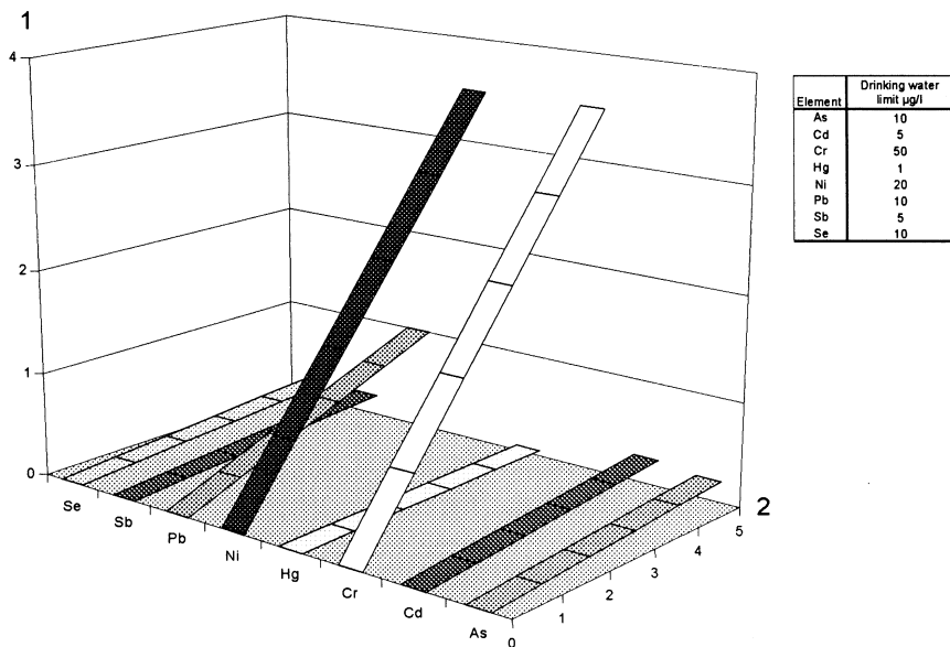
Figure A.1 — Maximum impact of aluminium iron (III) chloride (monomeric) and aluminium iron (III) chloride hydroxide (monomeric), type 1, on trace metal content of water
