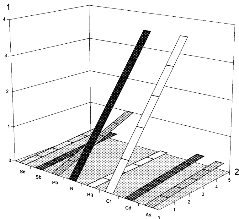
Figure A.1 — Maximum impact of aluminium salts, type 1, on trace metal content of water
