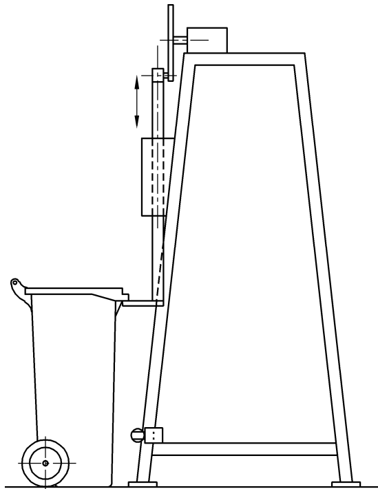
Figure B.1 — Apparatus for kerb fall test, 2-wheeled container
