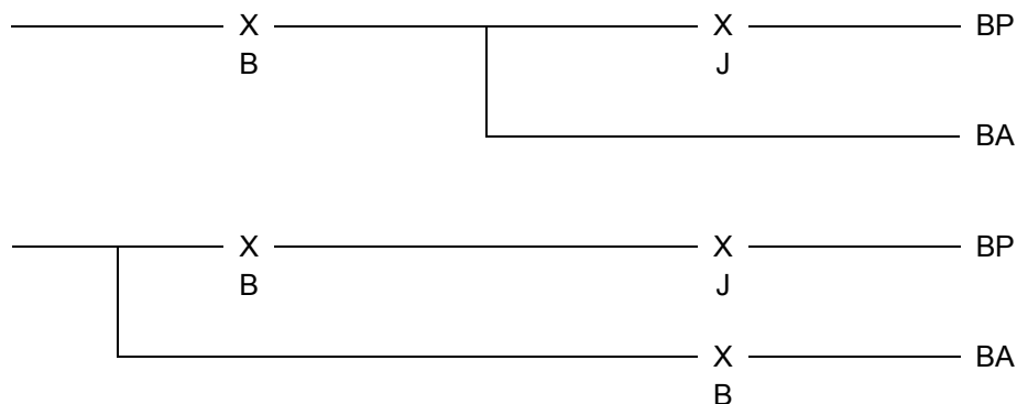
a) Systems with an ignition burner of heat input not exceeding 1 kW or 5 % of the main burner heat input
