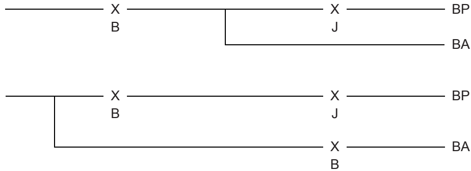
a) Systems with an ignition burner of heat input not exceeding 1 kW or 5 % of the main burner heat input
